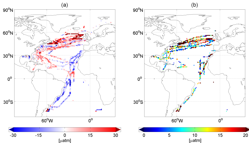
Fig. 1. (a) Temporal mean residuals and (b) standard deviation of the residuals in \mu\text{atm} between neural network estimates and independent data points obtained from the SOCAT v2 gridded observations.
