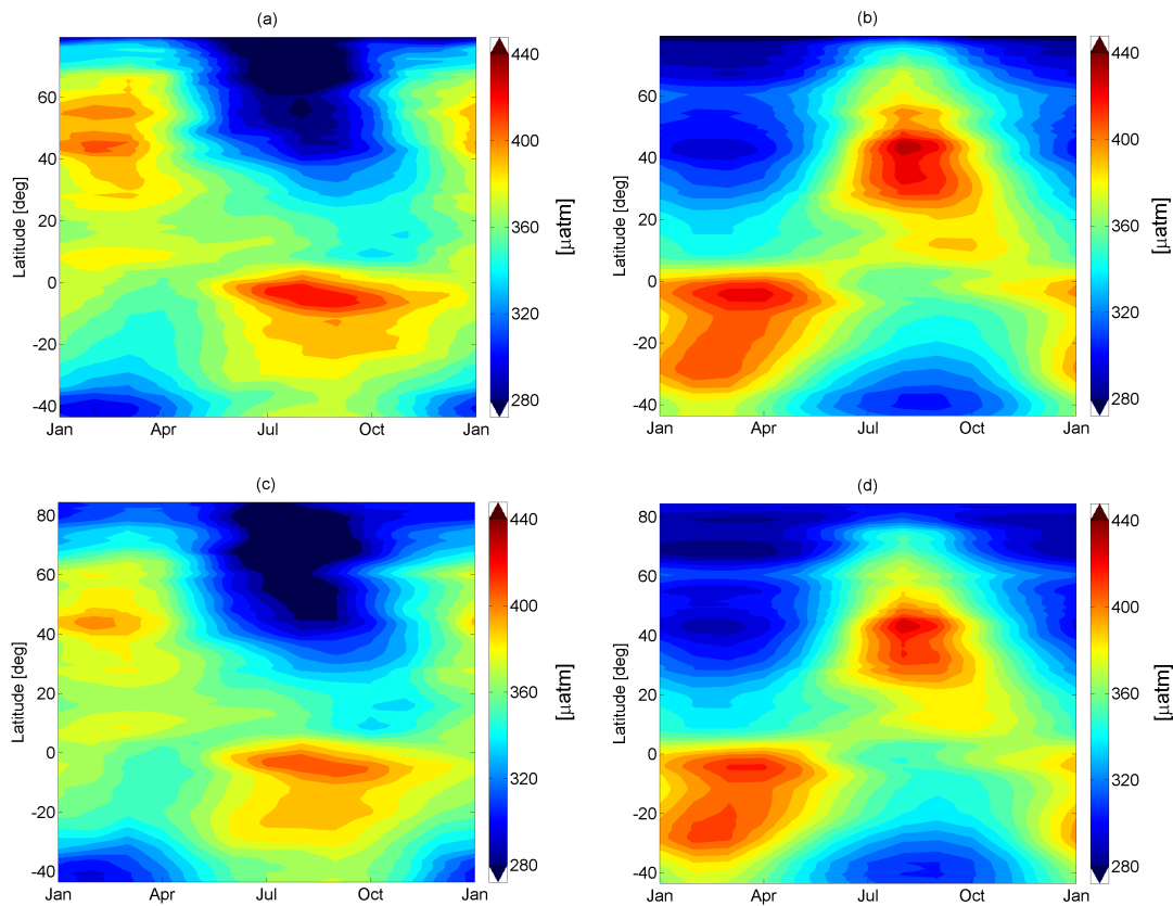
Fig. 2. ... Figure (c) and (d) show the non-thermal and thermal component respectively for the Takahashi et al. (2009) climatology. The decadal mean p\text{CO}_2 has been added to both components
