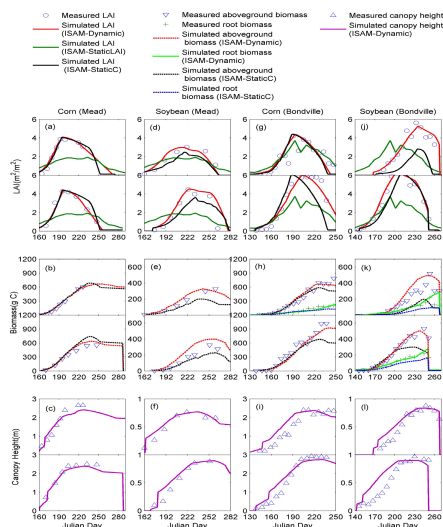
Figure 1. Measured and model simulated LAI, aboveground biomass, root biomass, canopy height under corn and soybean rotation at Mead and Bondville Ameri-Flux sites. Measured data for corn root biomass is available for the 2001 growing season and for soybean over the 2002 and 2004 growing seasons at Bondville, IL site. The top and the bottom panels for corn column are for 2001 and 2003 growing seasons, whereas for soybean column are for 2002 and 2004 growing seasons.
