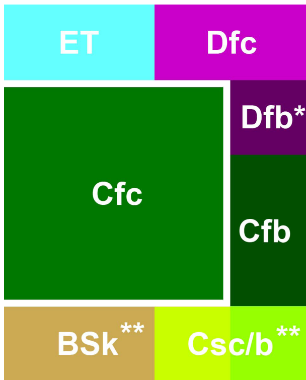
Fig. 1. Cfc Köppen climate type, typical of the coastal regions of modern Iceland, and its neighboring climate types. Note that plant taxa typical of a Cfc climate commonly occur at least in several further, adjacent climate types. (*) No direct contact, (**) direct contact only in Southern Hemisphere.
