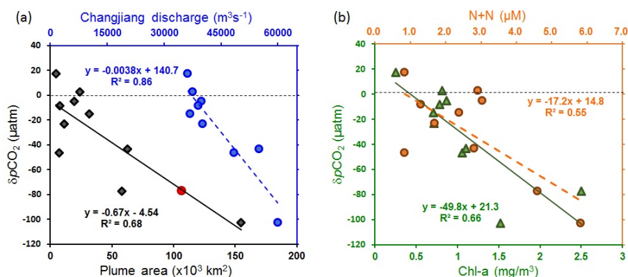
Fig. 1. Figure A-1. Relationships between the amounts of \delta p\text{CO}_2 and magnitudes of the CDW plume area and of the Changjiang discharge (a) and N+N and Chl-a (b) in summer from July 1998 to July 2011 in the ECS s
