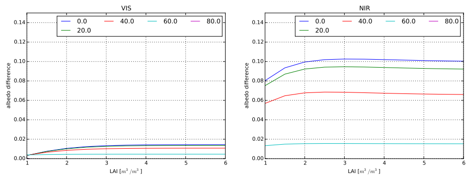
Fig. 1. Dependency of surface albedo difference \Delta \alpha on LAI for different sun zenith angles
