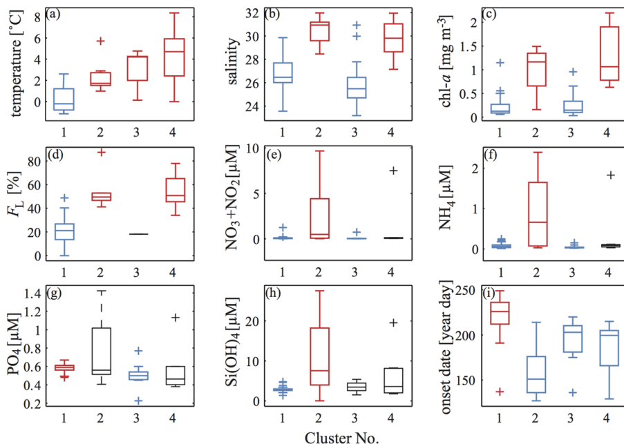
Fig. 6. Boxplots of (a) temperature, (b) salinity, (c) chl-a, (d) F_L , (e) \text{NO}_3 + \text{NO}_2 , (f) \text{NH}_4 , (g) \text{PO}_4 , (h) \text{Si(OH)}_4 and (i) onset date of sea ice retreat for the four clustered phytoplankton groups. Significant differences were detected by Steel-Dwass's multiple comparison test between blue and red plots. Plots of the same color and black plots are not significantly different. Note that the multiple comparison test was not conducted for F_L in cluster 3 because only one data point exists for that variable in that cluster.
