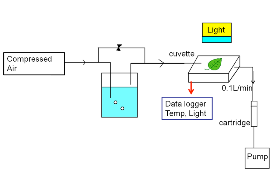
Fig. 2. A Schematic of the dynamic leaf enclosure cuvette set up.
