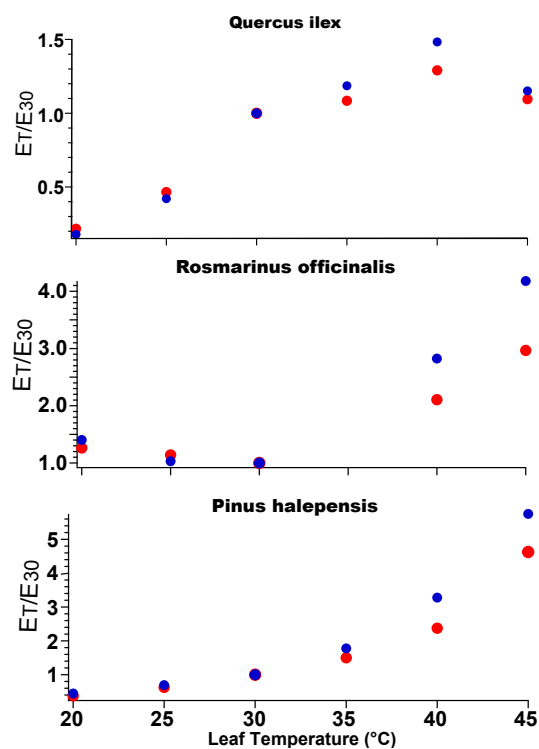
Fig. 6. An example of (-)/ (+)- \alpha -pinene emission which was normalized by dividing with emission at 30°C from different plant species in dependency with temperature.
