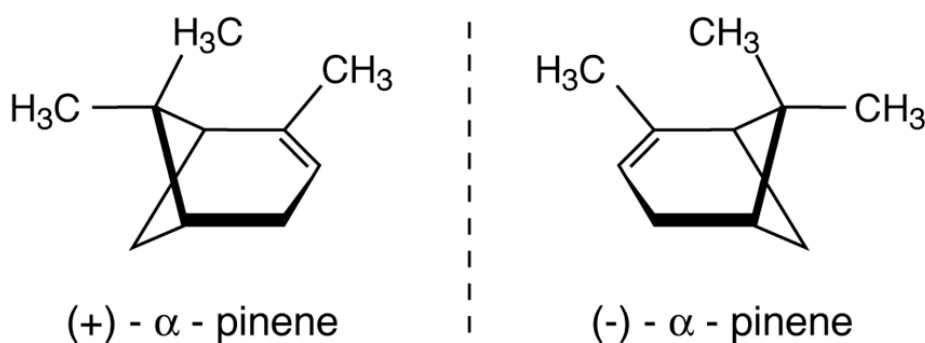
Fig. 1. Mirror image of α-pinene enantiomers.
