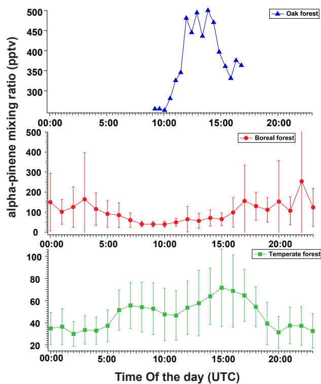
Fig. 8. Diel cycle of \alpha -pinene mixing ratios during the measurement period. For boreal forest and temperate forest measurements, the marks represent the mean value of every hour,
