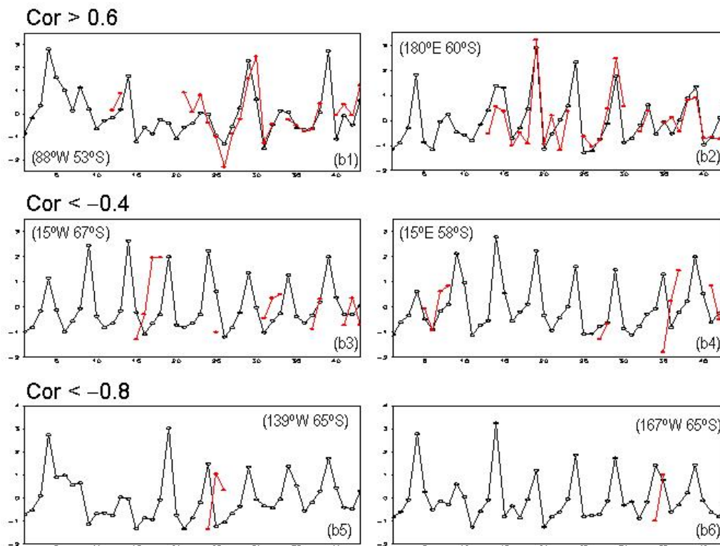
Fig. 2. Time series of Argo (red) and OFES (black) MLD at various grid points. Note that the labels along x-axis are in months. There are total 43 growing season months (Nov-Mar) between Jan 2001 and
