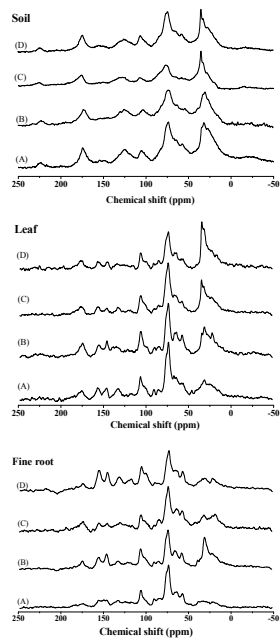
Figure 1. Solid-state ^{13}\text{C} CP/MAS NMR spectra for soil, leaf and fine root samples from four plantations in subtropical China: (A) Pinus massoniana , (B) Castanopsis hystrix , (C) Michelia macclurei and (D) Mytilaria laosensis .
