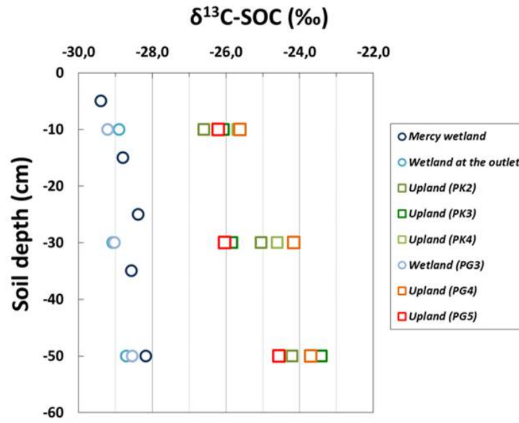
Fig. 3. Depth profile of \delta^{13}\text{C} for SOC from soils from the Kerolland (PK) and Gueriniec (PG) transects. Riparian soils are portrayed by circles, whereas squares refer to upland soils.
