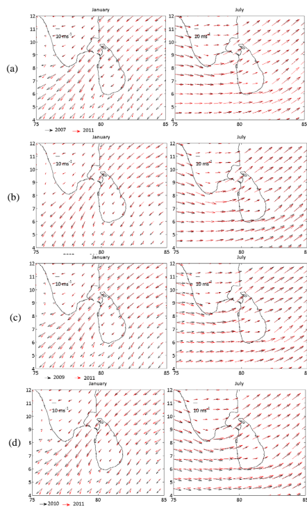
Fig. REF2.1 – Comparison of the wind fields from ECMWF ERA data during January (NE monsoon) and July (SW monsoon) to detect any significant changes in the wind during the La Nina year 2011. (a) comparison between 2007 and 2011; (b) comparison between 2008 and 2011; (c) comparison between 2009 and 2011; (d) comparison between 2010 and 2011.
