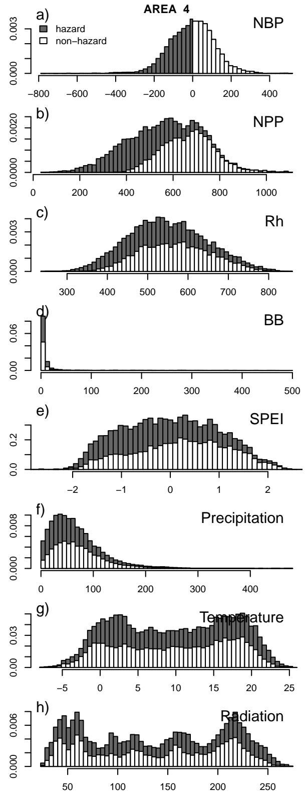
Fig. B5. Components of carbon fluxes in hazard and non-hazard group for area 4 (see Fig. B1).
