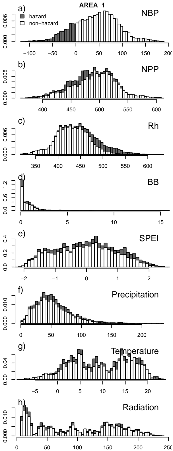
Fig. B2. Components of carbon fluxes in hazard and non-hazard group for area 1 (see Fig. B1).
