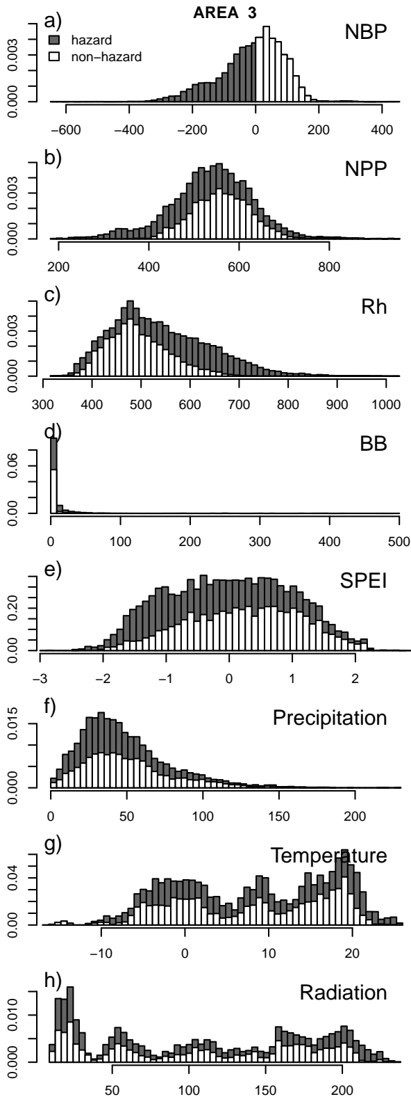
Fig. B4. Components of carbon fluxes in hazard and non-hazard group for area 3 (see Fig. B1).
