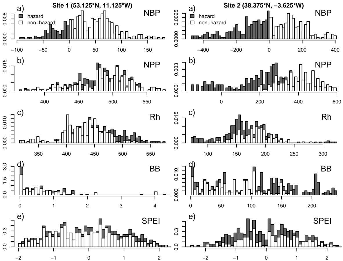
Fig. 3. Probability distributions of NBP (a) and its contributions NPP (b), Rh (c), and BB (d) (all in gC m -2 a -1 ) and SPEI values (e) for sites 1 (left) and 2 (right) (see Fig. 2). Dark shading denotes values in the hazard group, white shading in the non-hazard group.
