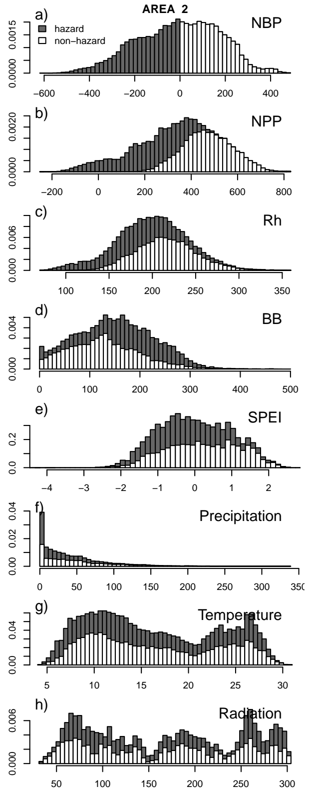
Fig. B3. Components of carbon fluxes in hazard and non-hazard group for area 2 (see Fig. B1).
