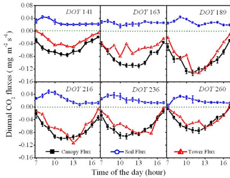
Fig. S1 Diurnal CO 2 flux measured at the soil surface, the plant canopy and the tower for six days in 2009.
