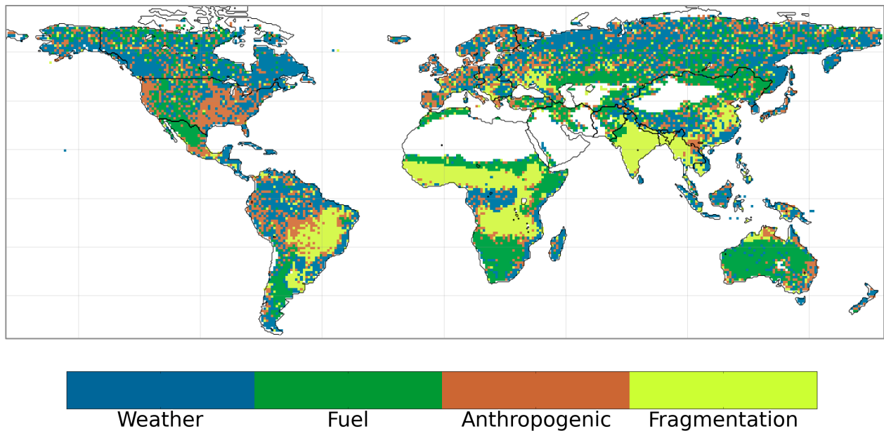
Figure 8. Major drivers of average annual burned area sensitivity among the 9 optimized parameters as grouped into 4 thematic classes (climate, vegetation fuel, anthropogenic practices, landscape fragmentation). For each of the 9 parameters, HESFIRE was run
