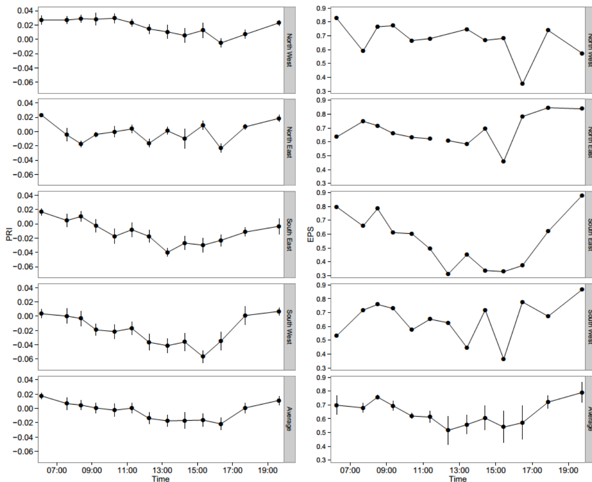
1 2 Fig. 9 Diurnal course of lodegopole pine ( Pinus contorta ) leaf-level photochemical reflectance 3 index (PRI) and the epoxidation state of the xanthophyll cycle components (EPS). PRI values for 4 each of the four directions are means of 10 sampled spectra. Error bars represent \pm 1 SEM.
