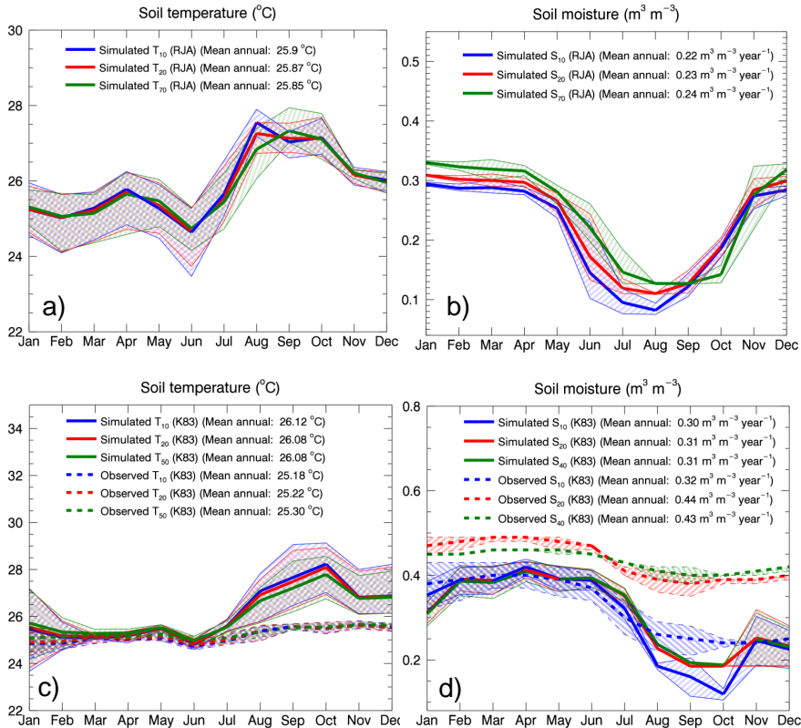
Figure 7. Simulated soil temperature ( a, c ) and soil moisture ( b, d ) at the RJA (Jarú Reserve) and K83 (Tapajós 83 km) sites. Observation-based soil temperature and moisture at K83 are also shown in ( c ) and ( d ) for soil depths given in cm .
