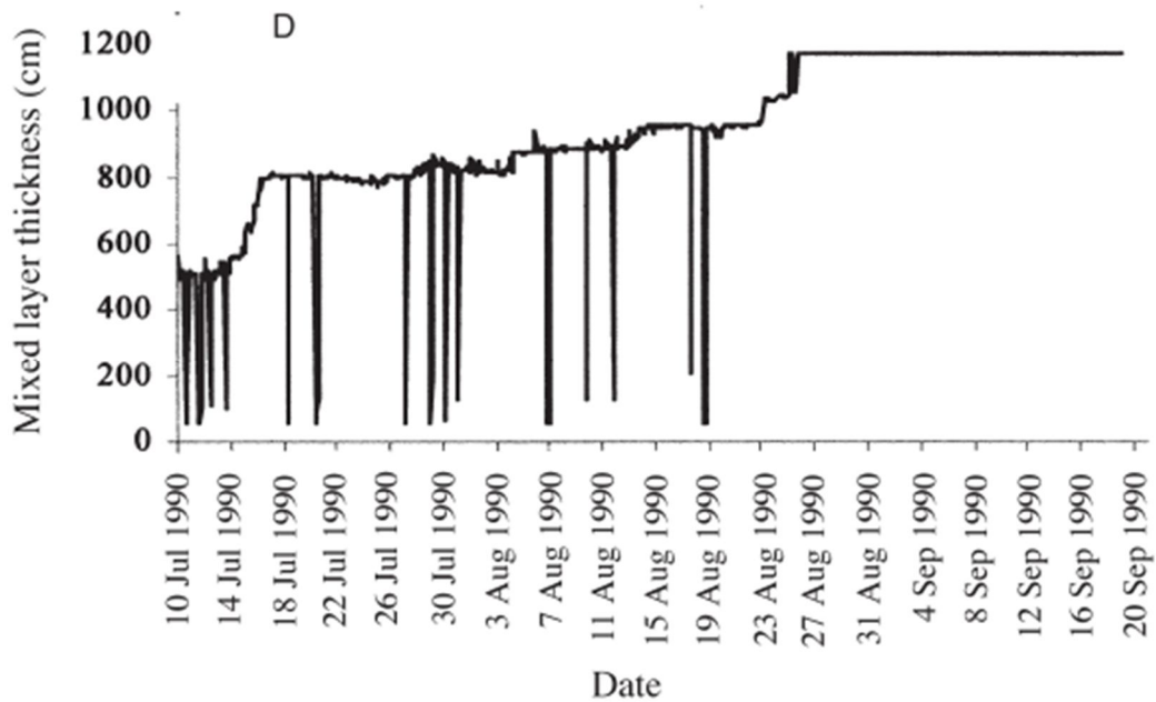
Fig 1.-Time series showing the mixed layer depth (in cm) in La Caldera Lake during the period July 10 to September 20, 1990 (from Rodriguez-Rodriguez et al., 2004)
