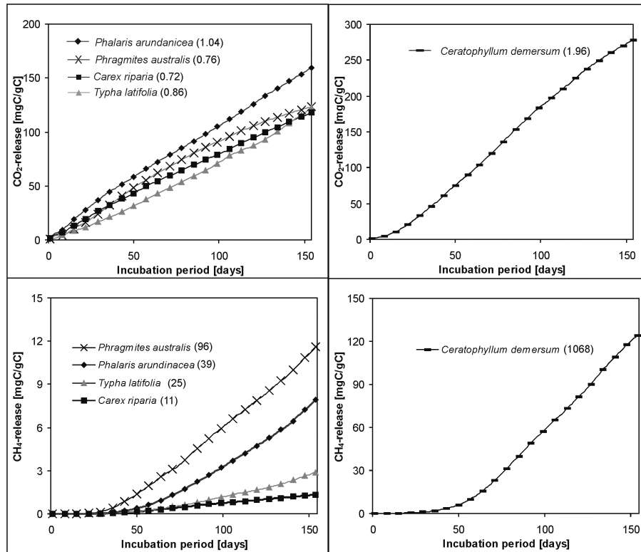
Figure 4. Cumulative release of \text{CO}_2 and \text{CH}_4 from different incubated plant material under submerged conditions over an incubation period over 154 d. The daily C-normalized gaseous C release is given in brackets (zero order rate constant: [k(\text{CO}_2)] = \text{mgC}(\text{d g C})^{-1} ; [k(\text{CH}_4)] \mu\text{gC}(\text{d g C})^{-1} calculated for day 40 to 154). Values are given as means ( n = 3 ). For better visualisation the cumulative values after always seven days are highlighted by symbols.
