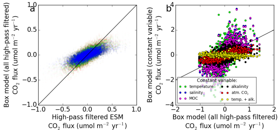
Fig. 7. Subpolar-North- a High-pass filtered ESPPE subpolar Atlantic surface-ocean-temperature-air-sea CO 2 flux plotted against box model estimates of that same flux using the top three box model parameter sets (table 2) in red, green and alkalinity-blue respectively, but forced with high-pass filtered input time-series. b All box model inputs high-pass filtered plotted from against all box model inputs high-pass filtered but one variable held constant. The constant variable in each case is named within the ESPPE simulations-legend. All results are presented as anomalies from their respective first 20 year the mean.
