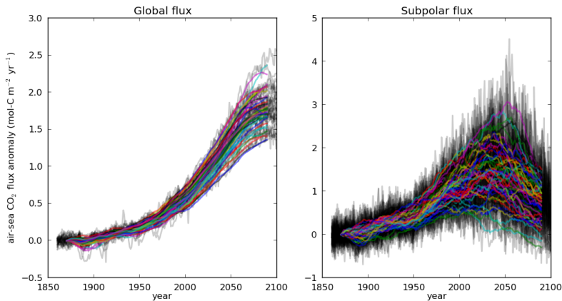
Fig. 1. Left: globally averaged air-sea CO 2 flux, and right: North Atlantic subpolar region averaged air-sea CO 2 flux. Black lines represent annually-averaged time series from all ESPPE members, and coloured lines represent those time series after application of a 20 year running mean.
