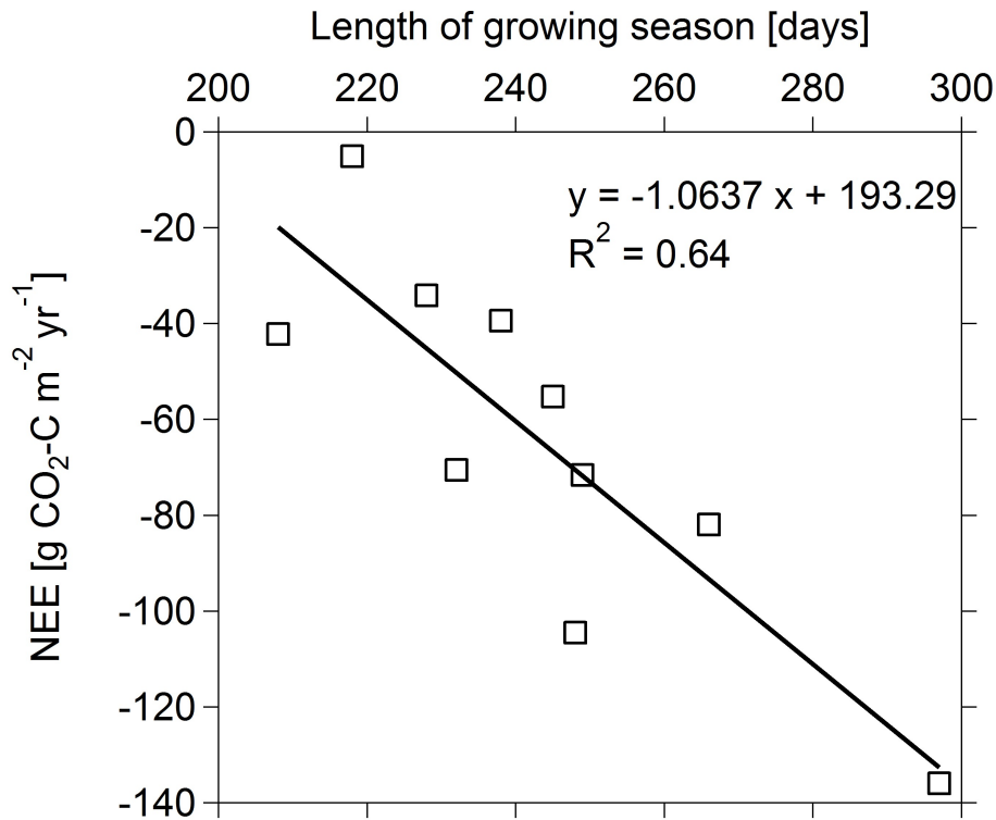
Figure 5. Annual NEE as a function of the length of the growing season.
