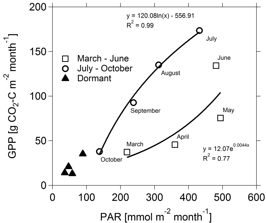
Figure 3. Hysteresis in gross primary production (GPP) as a function of photosynthetically active radiation (PAR) (10 year monthly means).
