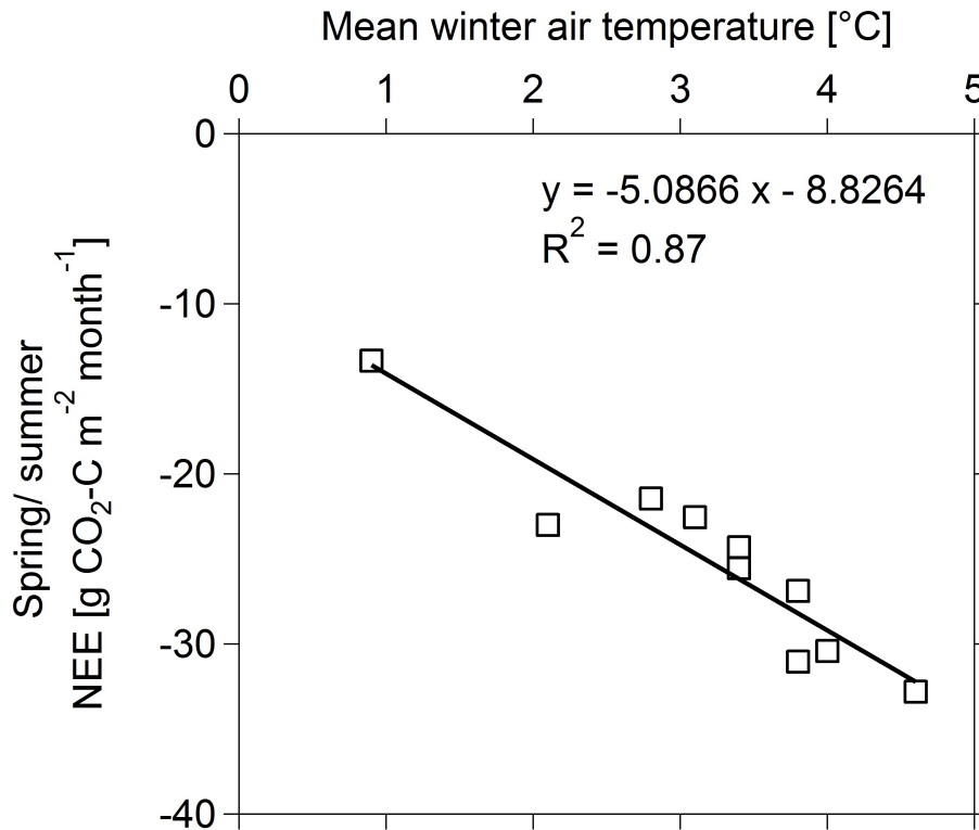
Figure 6. Spring/summer NEE (mean from April to September) as a function of the preceding winter's mean air temperature (mean from December to March).
