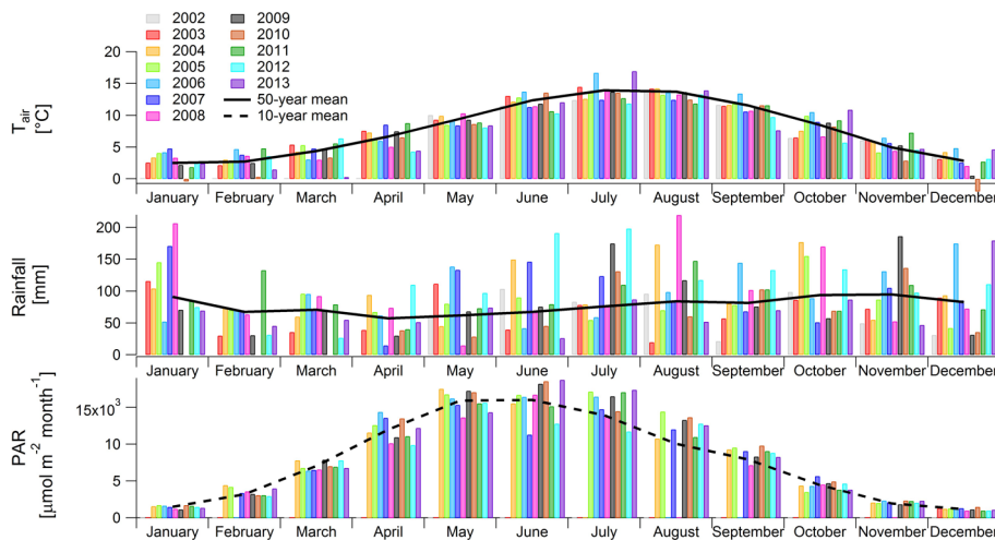
Figure 1. Monthly air temperature, rainfall and photosynthetically active radiation (PAR) for the study period 2002–2013.
