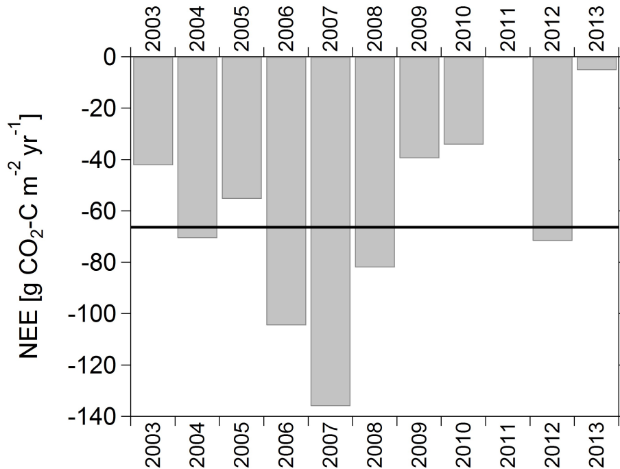
Figure 4. Annual NEE for 2003–2013 (no data for 2011 due to instrument failure during the growing season); the horizontal line is the mean NEE for the study period.
