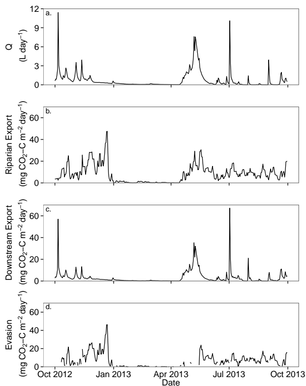
Figure 4. Mean daily a. discharge ( Q ), b. \text{CO}_2 export from the riparian zone to the stream, c. downstream lateral \text{CO}_2 export and d. vertical \text{CO}_2 evasion over the hydrological year.
