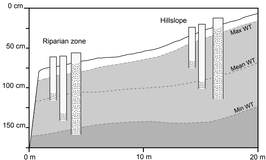
Figure 1. Schematic of the hillslope-riparian transect used in this study. CO 2 sensors were installed in dipwells with sampling windows at 30-40 cm and 60-70 cm depth. An additional dipwell for water table and soil temperature was perforated along the full length to 90 cm depth. Grey box indicates the zone of transient saturation (between max and min water table positions) over the hydrological year.
