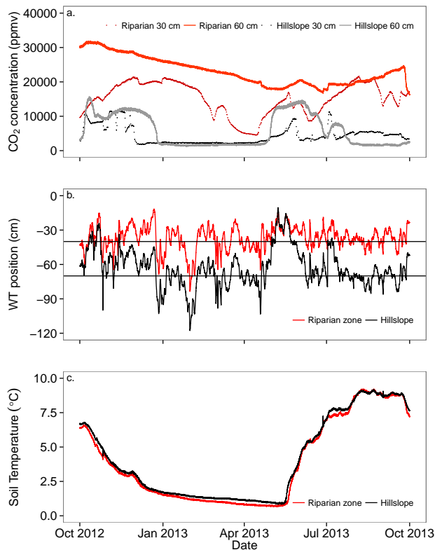
Figure 2. Time series of hillslope and riparian zone a. CO 2 concentrations sampled at 30-40 cm and 60-70 cm depths, b. water table and c. soil temperature across the full measurement period. Horizontal lines in b. highlight the deepest depths sampled by the 30-40 cm and 60-70 cm depth CO 2 sensors.
