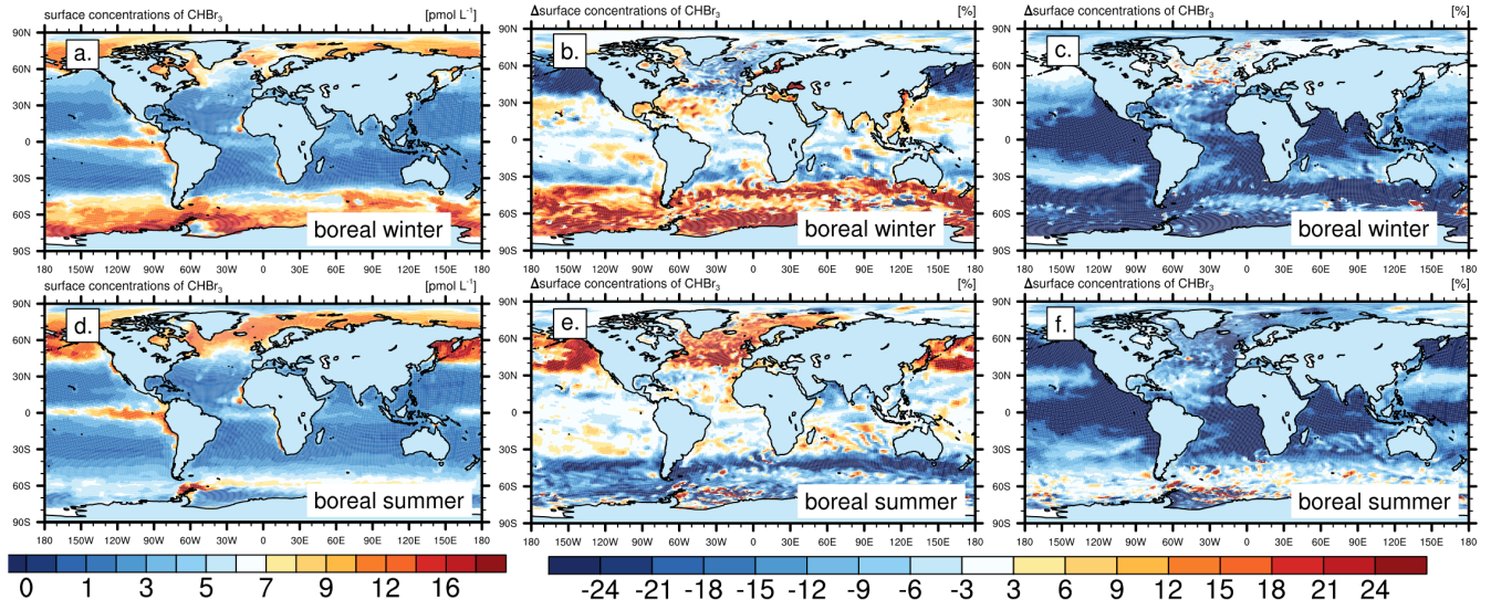
Figure 1: Mean surface bromoform concentrations ( \text{pmol L}^{-1} ) in experiment Ref in boreal winter (a) and boreal summer (d), percentage difference (e.g. 100 \cdot \frac{\text{Seas-at} - \text{Ref}}{\text{Ref}} ) of Seas-at (b, e) and Half (c, f) in the same season.
