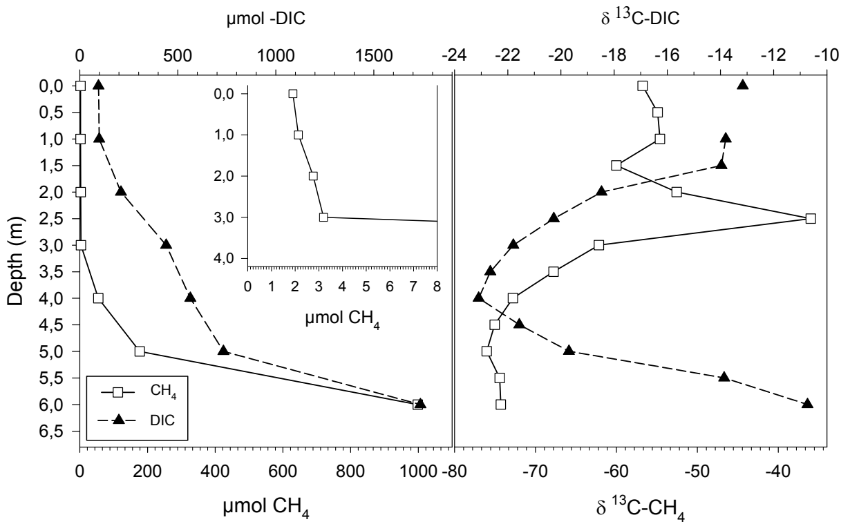
Supplementary Fig.1. Water column concentrations and \delta^{13}\text{C-CH}_4 for CH 4 (open box) and DIC concentrations and \delta^{13}\text{C} (filled triangles) on 27.8.2008, when sampling was with 0.5 m spacing. Superimposed insert shows CH 4 concentration in the upper water column.
