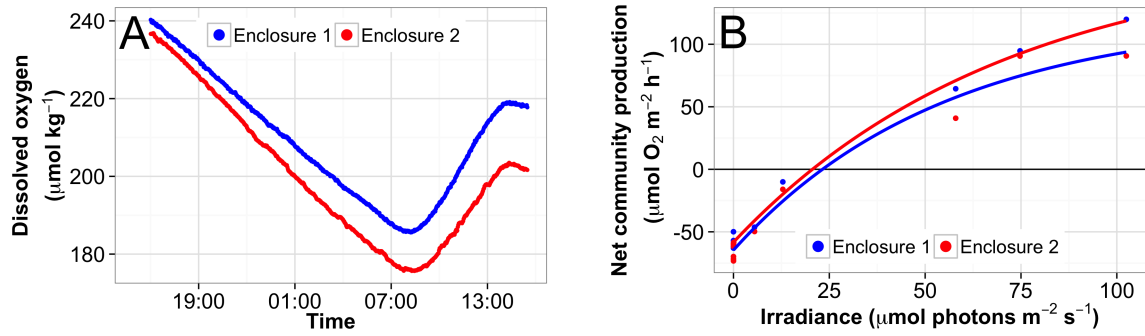
Fig. 3. Measurements of the community metabolism of a Posidonia seagrass bed in the northwest Mediterranean Sea performed in the frame of the eFOCE project. Oxygen variations (A) and photosynthesis-irradiance curves (B) during incubations performed in closed-chambers conditions.
