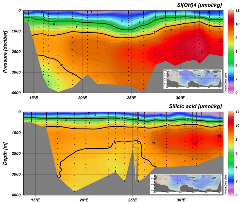
Fig. 2. X-section of Silicic acid from the Western Ionian Sea close to the location of Adriatic Deep Water formation in the Southern Adriatic to the Eastern Levantine Sea. Upper panel: X-section measured in 1987 and shows the Silicic acid distribution before the EMT increasing from 6.3 \mu\text{mol Si kg}^{-1} in the Western Ionian to 10.7 \mu\text{mol Si kg}^{-1} in the Eastern Levantine (data from Schlitzer et al., 1991 and Nellen et al., 1996) Lower panel: X-Section was measured in 1999 after EMT event and shows the presence of newer Deep water formed in the Aegean and advected into the deep water of the basin (data from Kress et al., 2003).
