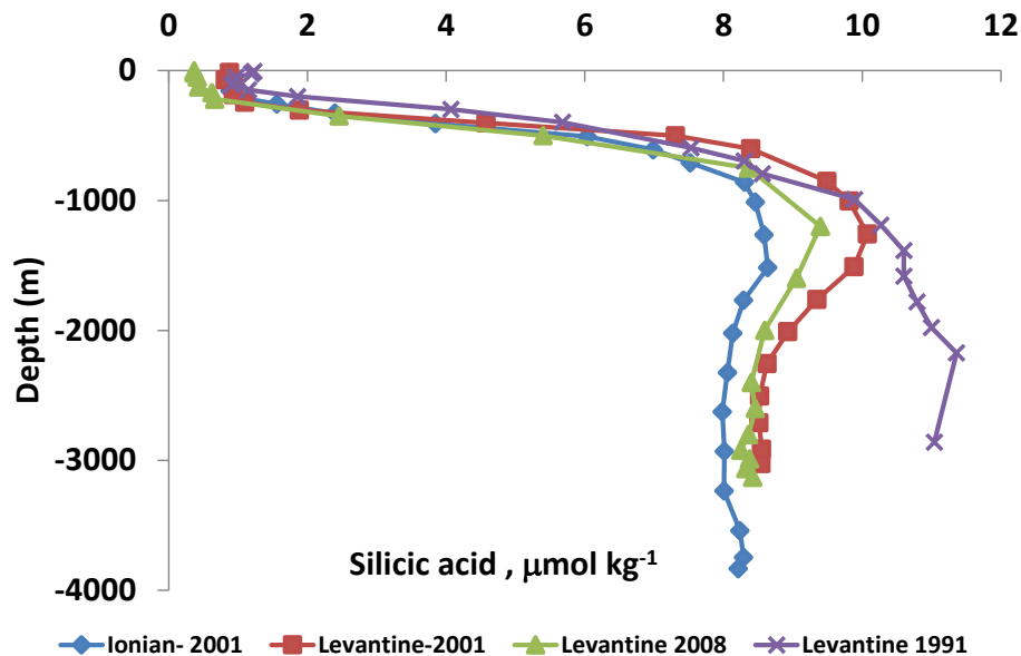
Fig. 1. Typical silicic acid profiles in the Levantine basin prior to the effect of the EMT event (1991), and after the EMT event (2001 and 2008). A profile in the Ionian (2001) is included for comparison. Data from Kress et al. (2003, 2014).
