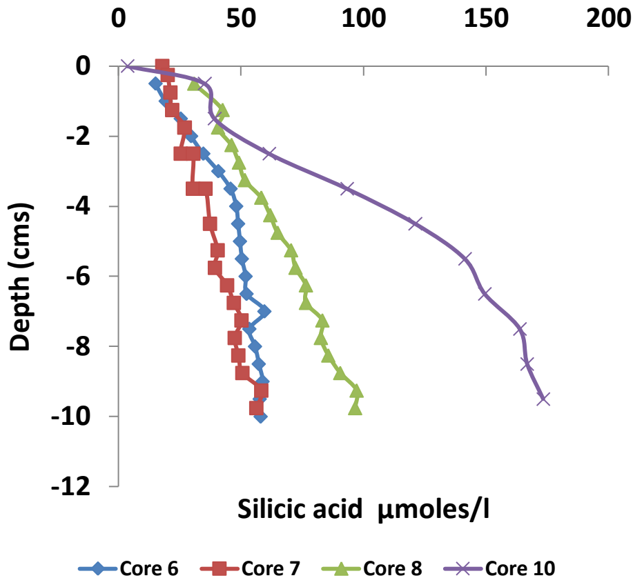
Fig. 3. Pore water profiles of silicic acid with depth from a series of pore water profiles in the deep water across the Eastern Mediterranean Sea sampled in 1975 (Jones, 1977).
