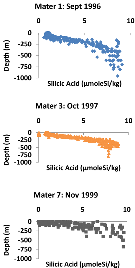
Fig. 4. Figure showing the vertical distribution of dissolved silicic acid in the water column of a series of stations across the Straits of Sicily sampled as part of the MTP-MATER programme (1996–1999). (Data from Lavezza et al., 2011.)
