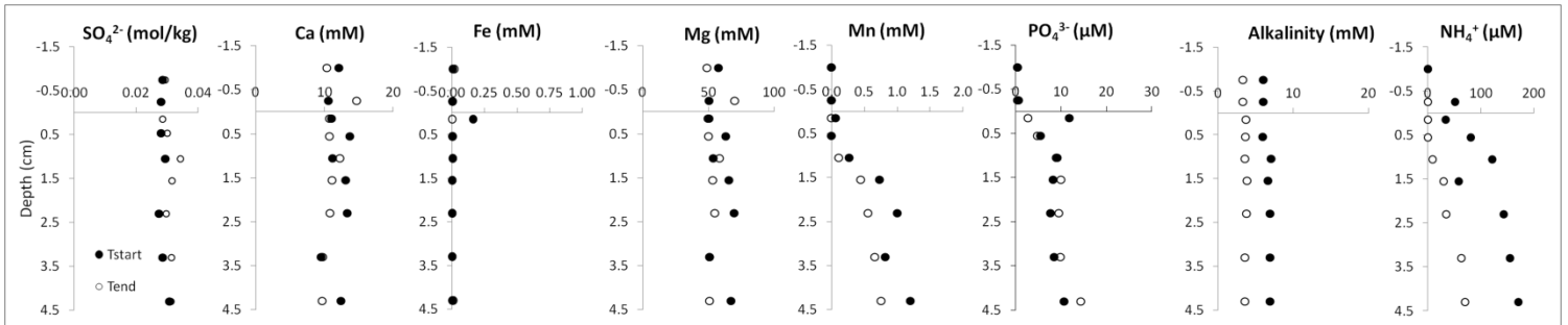
Figure A2. Element profiles for geochemical cores from experiment 2: B. marginata and C. laevigata . Please note that the scales for manganese, phosphates and ammonium are different from figure A1
