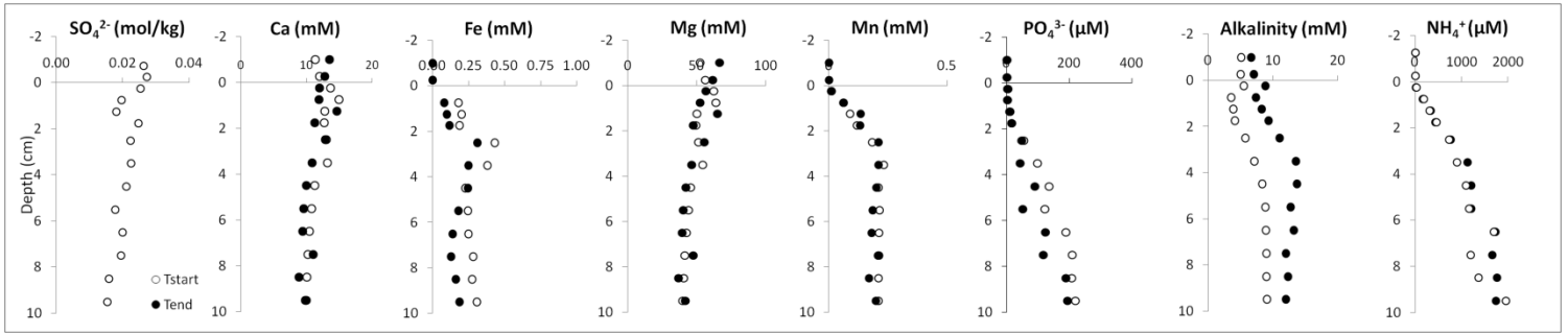
Figure A1. Element profiles for geochemical cores from Experiment 1: A. tepida
