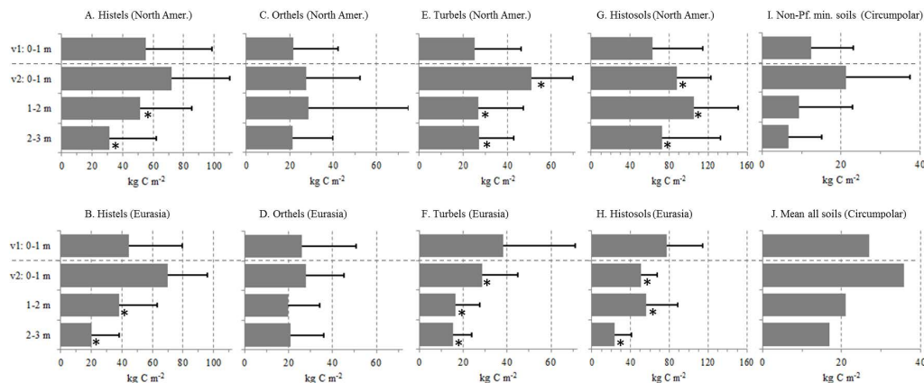
Fig. 3. Mean SOC storage ( \text{kg C m}^{-2} , with error bars showing StD), subdivided by continents, for different soil upscaling classes calculated using pedon datasets v1 and v2. Different panels (A) to (H) show estimates for the 0–1 m (pedon datasets v1 and v2), 1–2 m and 2–3 m (pedon dataset v2) depth ranges in the North American and Eurasian regions. Panel (I) shows estimated mean circumpolar SOC storage for all non-permafrost mineral soil orders (StD for v1 0–1 m is calculated from the StD of non-permafrost mineral soil orders in Table S1 of the Supplement, weighted for the total SOC mass of each soil order). Panel (J) shows circumpolar SOC storage estimated from the upscaled NCSCDv2 SOC stocks, as calculated with the two pedon datasets. Asterisks mark depth intervals in soil upscaling classes where SOC storage is significantly different from the equivalent interval in the other region ( t test, p < 0.05 ).
