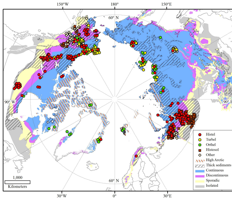
Fig. 1. Geographical distribution of regions with thick sedimentary overburden and permafrost zonation in the northern circumpolar permafrost region (Brown et al., 2002). Map shows pedon locations with data in the 0–3 m depth range (pedon dataset v2) grouped according to NCSCDV2 upscaling classes. Exact pedon locations have been manipulated for cartographic representation; projection: Azimuthal Equidistant, datum: WGS84. Adapted from Hugelius et al. (2013a).
