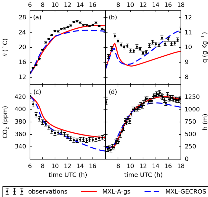
Figure 4. Daytime diurnal cycle of (a) the potential temperature \theta , (b) the specific humidity q , (c) the \text{CO}_2 mole fraction and (d) the boundary-layer height h , at the maize site, on the 4 August 2007. The errors for the \theta , q and \text{CO}_2 measurements are obtained based on the factory specifications of the instruments. The error for h is assumed to be constant and equal to 50 m (personal communication, Henk Klein Baltink). Note that, in order to reproduce the early morning temperature and humidity variations, we prescribed advection of heat until 10:00 UTC and advection of humidity until 07:30 UTC (see settings in Table A1).
