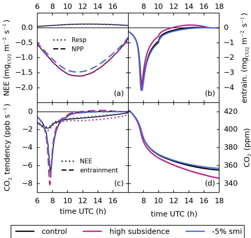
Figure 9. Contributions of the surface and entrainment fluxes to the atmospheric \text{CO}_2 budget. Net photosynthesis (NPP) and soil respiration (Resp) combine at the surface to form NEE, while the entrainment of \text{CO}_2 (entrain.) takes place at top of the boundary layer. All these fluxes are negative when \text{CO}_2 is being removed from the boundary layer. The \text{CO}_2 tendencies, which determine the daytime diurnal cycle of \text{CO}_2 , are obtained by dividing these \text{CO}_2 fluxes by the instantaneous boundary-layer height.
