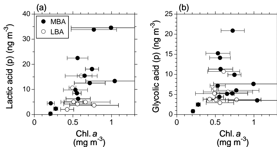
Fig. 3. Concentrations of (a) lactic and (b) glycolic acids in the particulate phase as a function of chlorophyll a concentrations in seawater for more biologically influenced aerosols (MBA) and less biologically influenced aerosols (LBA).
