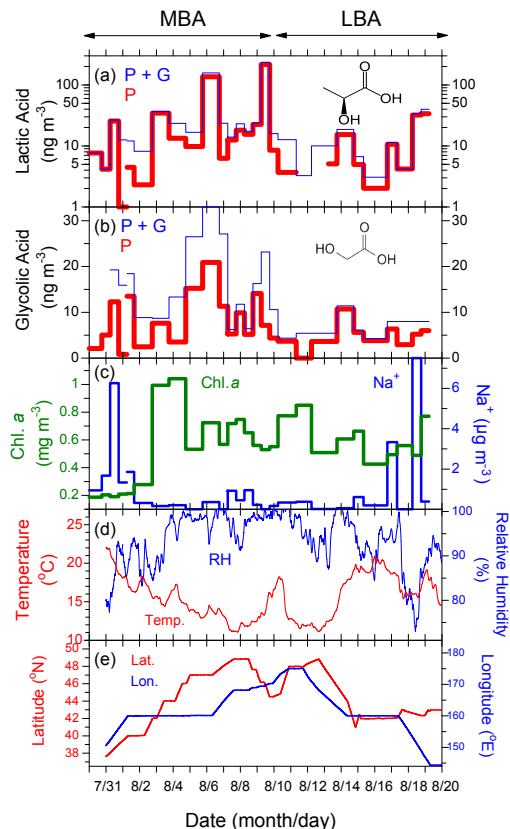
Fig. 1. Time series of the concentrations of (a) lactic acid and (b) glycolic acid in the particle ( p ) phase and the sum of gas and particle ( g + p ) phases, (c) chlorophyll a concentrations in sea water and \text{Na}^+ concentrations in aerosols, (d) ambient temperature and relative humidity, and (e) the ship position (latitude and longitude) during the R/V Hakuho-Maru cruise. See the text for the definition of MBA (30 July–7 August 2008) and LBA (9–19 August 2008) periods. The y-axis of (a) is plotted on a log scale.
