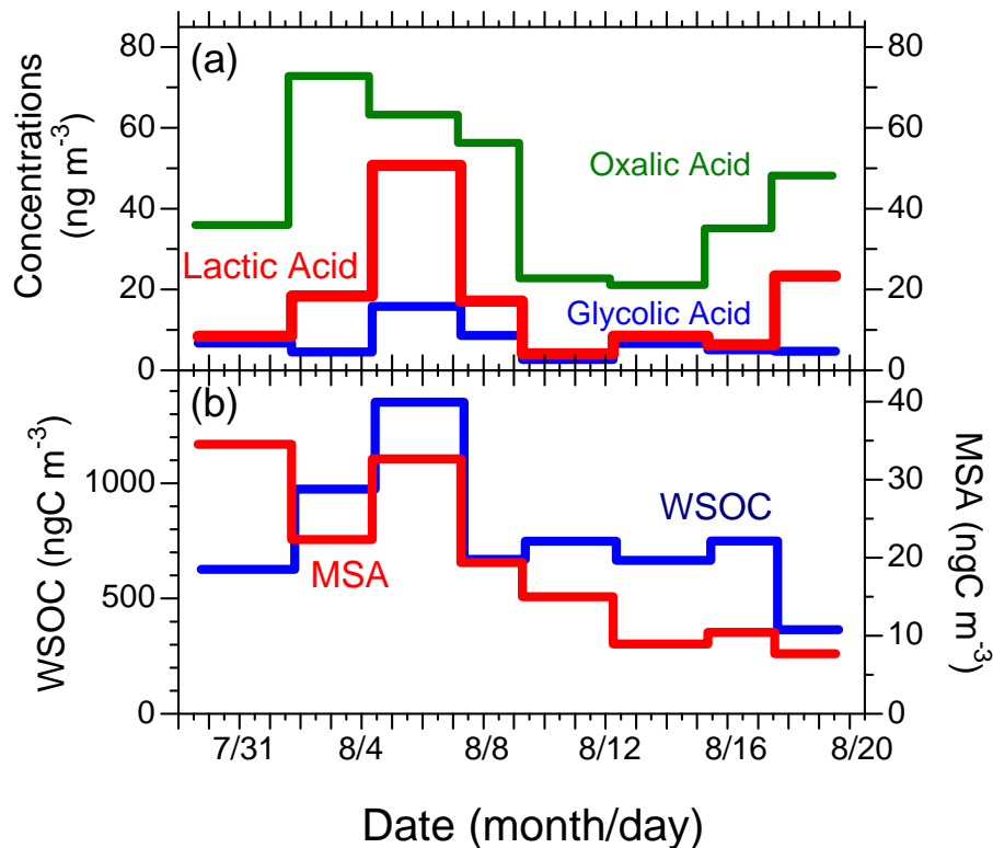
Fig. 2. Time series of the concentrations of (a) lactic acid (LA) and glycolic acid (GA) in the particle phase compared with those of oxalic acid, (b) water-soluble organic carbon (WSOC), and methanesulfonic acid (MSA). The duration of LA and GA measurements was averaged over that of oxalic acid, WSOC, and MSA; measurements were performed with a cascade impactor every 2–3 days.
