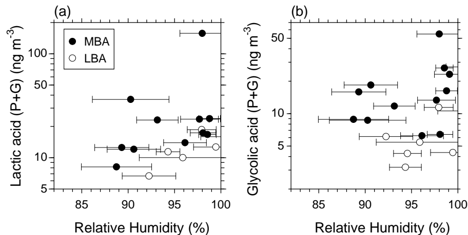
Fig. 4. Concentrations of (a) lactic and (b) glycolic acids in the gas and particle ( g + p ) phases as a function of relative humidity for MBA and LBA. The y-axis is plotted on a log scale.
