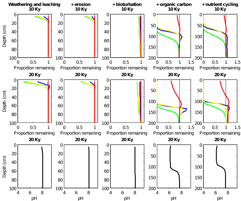
Fig. 3. Vertical distributions of pH and the relative depletion/enrichment of the basic model oxides over 20kyr of soil development for five different model runs of increasing complexity. Values <1 indicate a loss relative to the parent material, and values >1 indicate relative accumulation.
