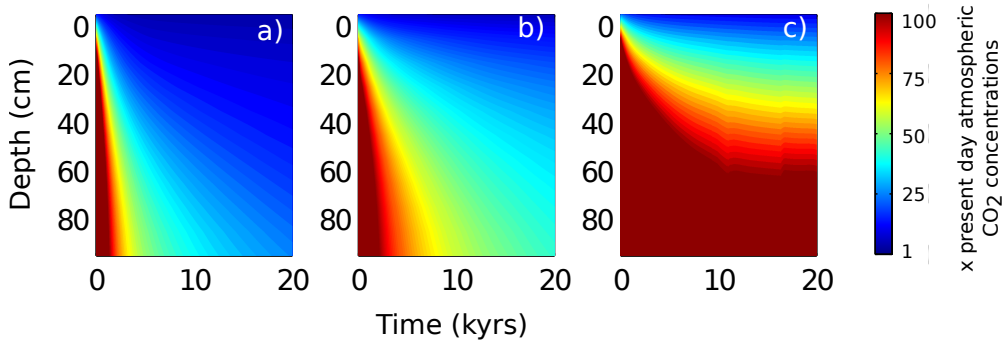
Fig. 9. Evolution of CO 2 profiles over 20 kyrs of soil development for three different model scenarios. N_P=0.5 \text{ kg m}^{-2} \text{ yr}^{-1} and z_r=0.26 (a), N_P=1 \text{ kg m}^{-2} \text{ yr}^{-1} and z_r=0.26 (b) and N_P=1 \text{ kg m}^{-2} \text{ yr}^{-1} and z_r=0.5 (c).
