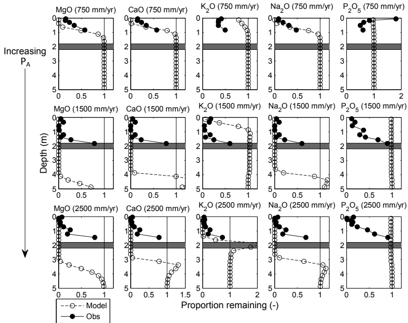
Fig. 14. Observed vs. simulated oxide losses/gains across a mean annual precipitation gradient ( P_A ) on the 350ka Pololu lava flow. Values <1 indicate a loss relative to the parent material, and values >1 indicate relative accumulation. The grey box shows the location of the pahoehoe flow.
