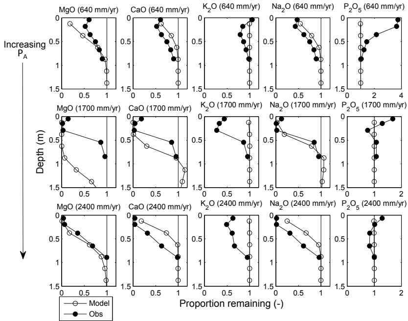
Fig. 11. Observed vs. simulated oxide losses/gains across a mean annual precipitation gradient ( P_A ) on the 10ka Kona lava flow. Values <1 indicate a loss relative to the parent material, and values >1 indicate relative accumulation.
