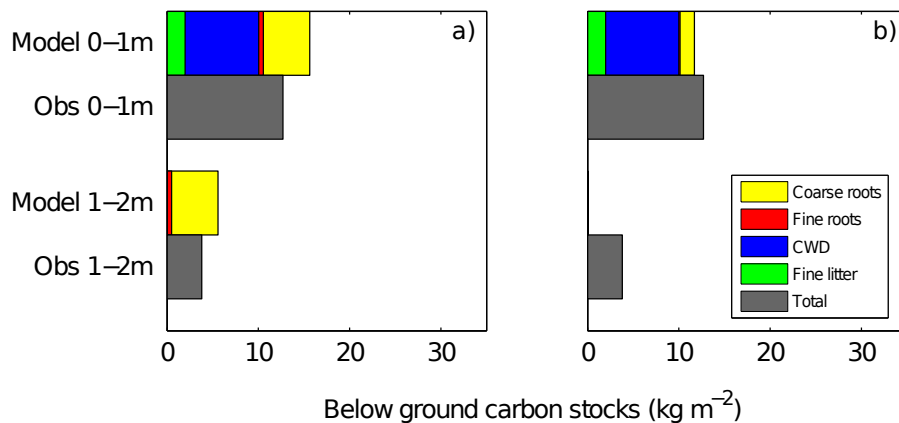
Fig. 7. Steady-state distribution of organic carbon pools for a) the control run (Table 1) and b) a constant decay rate with soil depth. Observations are from the Manaus site in Malhi et al. (2009). The total N_P for both runs is the same as the previous simulations which is equal to that estimated by Malhi et al. (2009) for the Manaus forest plot (Table 1).
