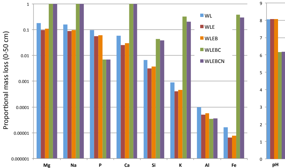
Fig. 5. Proportional mass loss of each model element relative to the amount in the parent material and mean pH for the top 50 cm of the soil profile after 20 kyr of soil development for each of the model simulations (WL = weathering and leaching, E = erosion, B = bioturbation, C = organic carbon and N = nutrient cycling).
