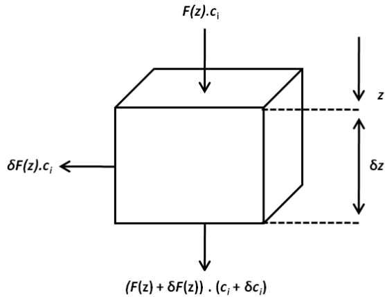
Fig. 2. Schematic overview of solute mass balance where F is the rate of percolation ( \text{m yr}^{-1} ) at depth z and c is the concentration of ion i in solution ( \text{g m}^{-3} ). Adapted from Kirkby (1985)
