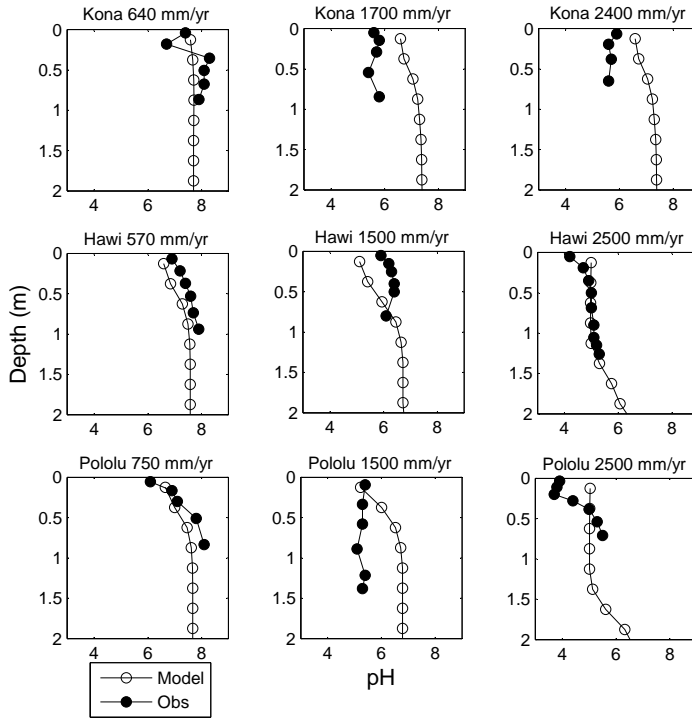
Fig. 15. Observed vs. simulated pH for 3 sites on each of the lava flows.
