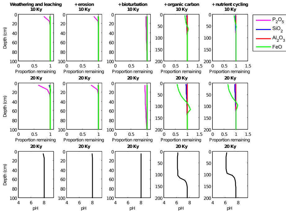
Fig. 4. Vertical distributions of pH the relative depletion/enrichment of the non-basic model oxides over 20kyr of soil development for five different model runs of increasing complexity. Values <1 indicate a loss relative to the parent material, and values >1 indicate relative accumulation.
