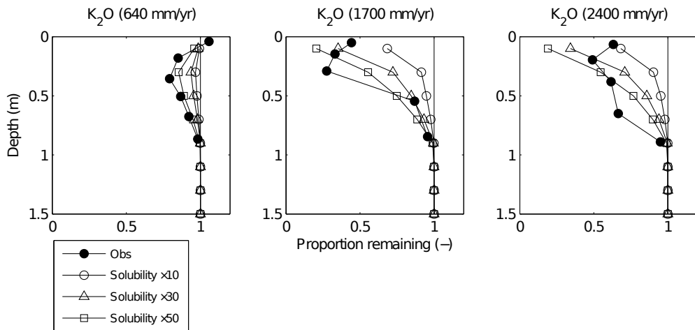
Fig. 12. Observed vs. simulated K for the 10ka Kona flow for 3 different simulations of increased K solubility.
