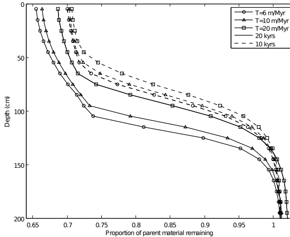
Fig. 6. Proportion of original parent material remaining after 10 and 20 kyr of model simulation for 3 different rates of surface erosion ( T ).
