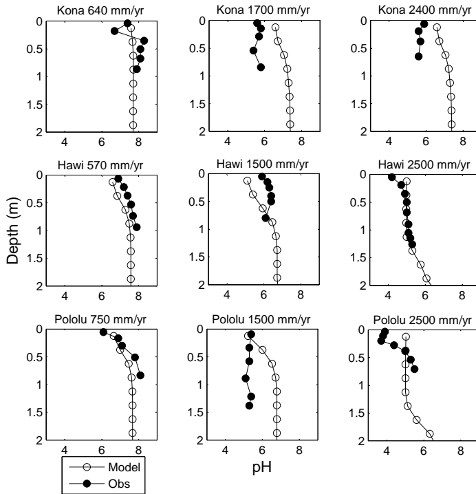
Fig. 12. Observed vs. simulated pH for 3 sites on each of the lava flows.
