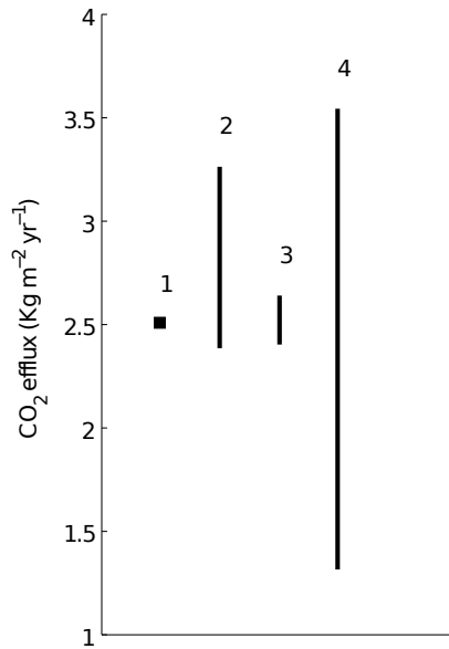
Fig. 7. Modelled soil respiration rate after 20 kyrs of soil development (1) and ranges of measured soil respiration rates from the following studies of Hawaiian tropical soils 2.Raich (1998) 3.Townsend et al. (1995) 4.Schuur and Matson (2001).
