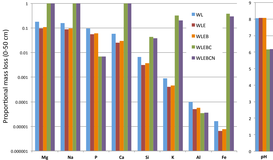
Fig. 4. Proportional mass loss of each model element relative to the amount in the parent material and mean pH for the top 50 cm of the soil profile after 20 kyr of soil development for each of the model simulations (WL = weathering and leaching, E = erosion, B = bioturbation, C = organic carbon and N = nutrient cycling).
