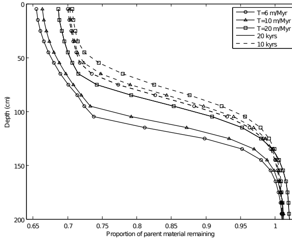
Fig. 5. Proportion of original parent material remaining after 10 and 20 kyr of model simulation for 3 different rates of surface erosion ( T ).
