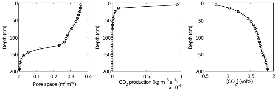
Fig. 6. Profiles of pore space ( 1-p ), \text{CO}_2 production rate and \text{CO}_2 concentration after 20 kyrs of soil development.
