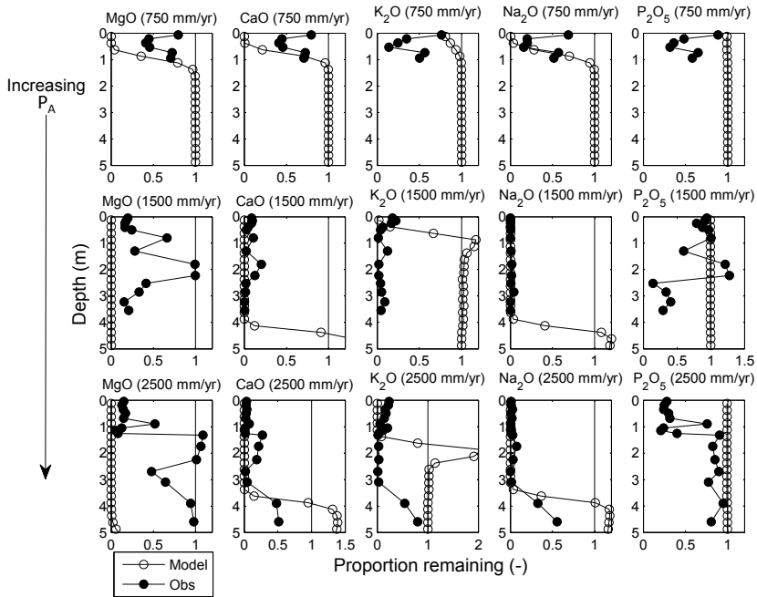
Fig. 10. Observed vs. simulated oxide losses/gains across a mean annual precipitation gradient ( P_A ) on the 170ka Hawi lava flow. Values < 1 indicate a loss relative to the parent material, and values > 1 indicate relative accumulation.
