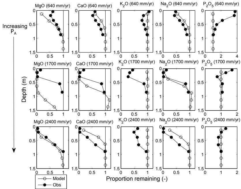
Fig. 8. Observed vs. simulated oxide losses/gains across a mean annual precipitation gradient ( P_A ) on the 10ka Kona lava flow. Values <1 indicate a loss relative to the parent material, and values >1 indicate relative accumulation.
