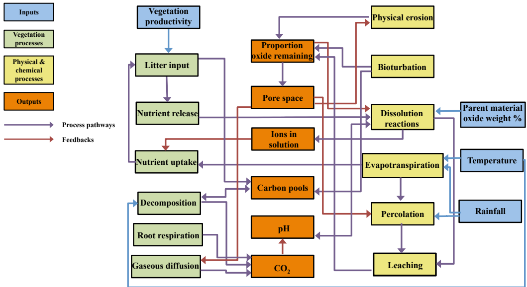
Fig. 2. Diagram of the major processes, inputs and outputs of the soil profile model
