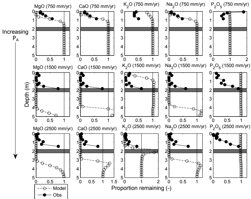
Fig. 11. Observed vs. simulated oxide losses/gains across a mean annual precipitation gradient ( P_A ) on the 350ka Pololu lava flow. Values <1 indicate a loss relative to the parent material, and values >1 indicate relative accumulation. The grey box shows the location of the pahoehoe flow.
