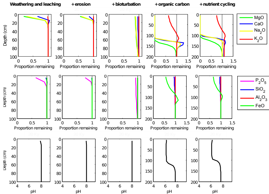
Fig. 3. Vertical distributions of pH and the relative depletion/enrichment of the elemental model oxides after 20kyr of soil development for five different model runs of increasing complexity. Values < 1 indicate a loss relative to the parent material, and values > 1 indicate relative accumulation.
