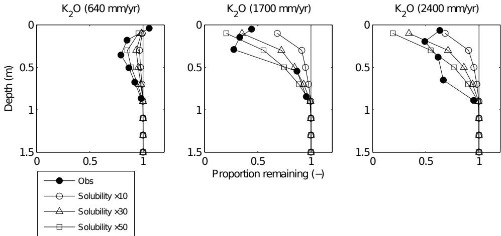
Fig. 9. Observed vs. simulated K for the 10ka Kona flow for 3 different simulations of increased K solubility.
