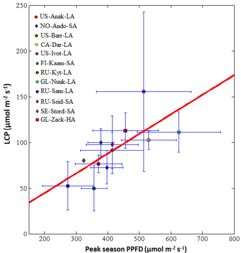
Fig. 6. Averaged peak season PPFD (light) control on light compensation point (LCP) parameter. r^2 = 0.5 , p = 0.008 . Ecosystems in regions prone to high light tend to be adapted to such conditions with a correspondingly high LCP.
