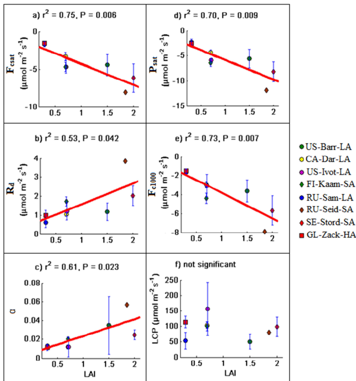
Fig. 2. Relationships between maximum leaf are index (LAI) and (a) light saturation NEE, F_{csat} ; (b) dark respiration, R_d ; (c) rate of carbon assimilation with initial increase in light, \alpha ; (d) potential photosynthesis at light saturation, P_{sat} ; (e) NEE when PPFD is 1000 \mu\text{mol m}^{-2} \text{s}^{-1} , F_{c1000} and (f) light compensation point (LCP). Red line represents linear fit between maximum LAI and LRC parameters while error bars are standard deviations.
