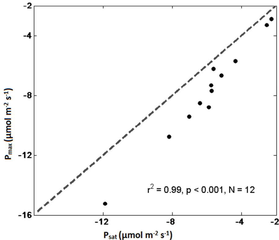
Fig. B3. Correlations between Eq. (1) (Falge et al., 2001) and (2) (Ruimy et al., 1995) using photosynthesis at light saturation. Potential photosynthesis at light saturation ( P_{\text{sat}} ) was calculated as the sum of F_{\text{csat}} and R_{\text{d}} in Eq. (1) (Falge et al., 2001; Lindroth et al., 2007) and was estimated by P_{\text{max}} in Eq. (2) (Frolking et al., 1998; Laurila et al., 2001; Ruimy et al., 1995) based on the 12 sites in this study. Broken line represents the 1 : 1 line.
