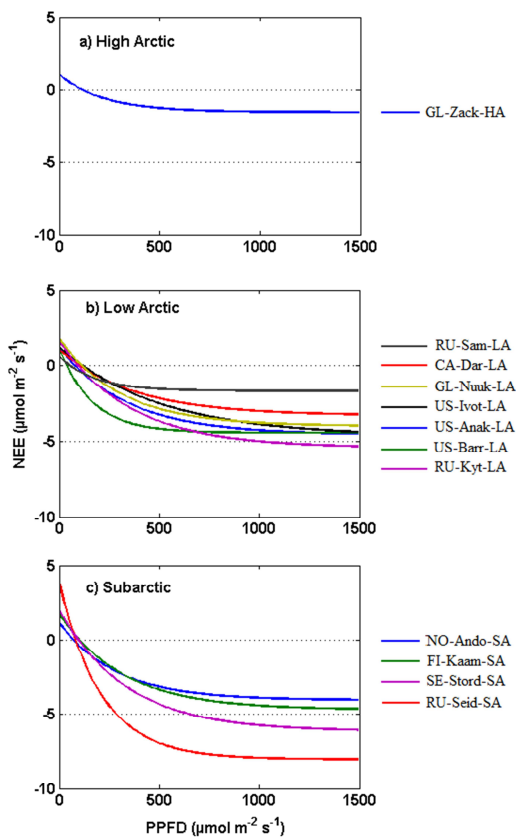
Fig. 4. Light response curves across the Arctic tundra, (a) High Arctic sites, (b) Low Arctic sites, (c) Subarctic sites. Classification was done according to Arctic floristic boundaries (AMAP, 1998)
