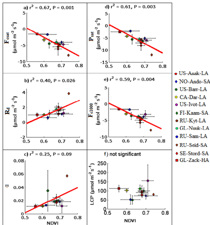
Fig. 3. Relationships between peak season NDVI and (a) light saturation NEE, F_{csat} ; (b) dark respiration, R_d ; (c) rate of carbon assimilation with initial increase in light, \alpha ; (d) potential photosynthesis at light saturation, P_{sat} ; (e) NEE when PPFD is 1000 \mu\text{mol m}^{-2} \text{s}^{-1} , F_{c1000} and (f) light compensation point (LCP). Red line represents linear fit between peak season NDVI and LRC parameters while error bars are standard deviations.
