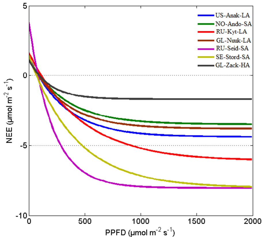
Fig. B4. Comparing LRC curves for peak period 2008 shows that F_{\text{csat}} for RU-Seid-SA may be comparable to SE-Stord-SA but differs in terms of \alpha and R_d . Also, the LRC for RU-Seid-SA shows a stronger and unique curvature.
