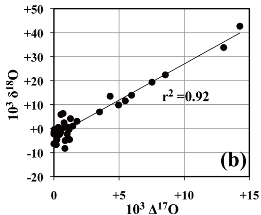
Figure 4. Relationship between \Delta^{17}\text{O} and \delta^{15}\text{N} of nitrate (a) and \Delta^{17}\text{O} and \delta^{18}\text{O} of nitrate (b) in stream water samples.
