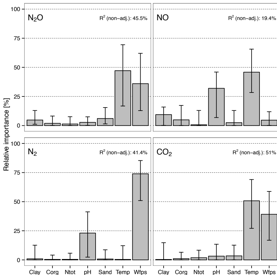
Figure 6. Relative importance of environmental factors clay, organic carbon (Corg), total nitrogen (Ntot), sand, temperature and water filled pore space (Wfps) on N_2O , NO , N_2 and CO_2 emissions (based on proportional marginal variance decomposition, R^2 values give total predictability of each model).
