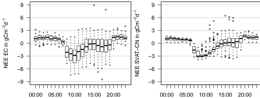
Figure C3. Mean diel course of measured (left panel) and modelled (tile approach according to the EC footprint: S_{\text{RefEC}} , right panel) net ecosystem exchange (NEE) over 61 days of 2010 (3 June to 2 August) at Kema: box plot with median, 25% and 75% quartiles; bars represent quartiles \pm 1.5 times interquartile range, dots are outliers. Measured and modelled values are restricted to high data quality (flag 1–3 out of a scheme ranging from 1–9, Foken et al., 2004).
