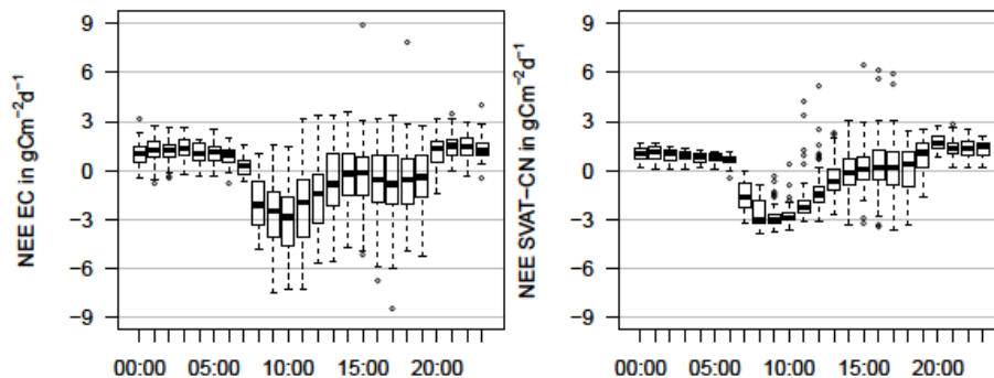
Figure D3. Mean diel course of measured (left panel) and modelled (tile approach according to the EC footprint: S_{\text{RefEC}} , right panel) net ecosystem exchange (NEE) over 61 days of 2010 (3 June to 2 August) at Kema: box plot with median, 25 % and 75 % quartiles; bars represent quartiles \pm 1.5 times interquartile range, dots are outliers. Measured and modelled values are restricted to high data quality (flag 1–3 out of a scheme ranging from 1–9, Foken et al., 2004).
