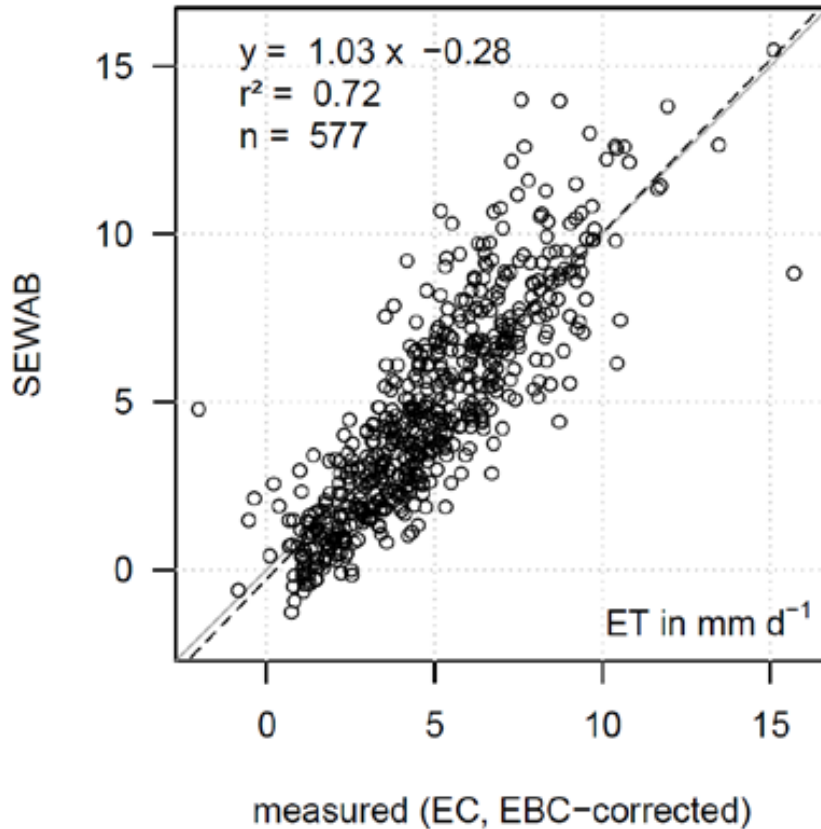
Figure D1. Scatterplot of measured vs. SEWAB modelled S_{\text{RefEC}} evapotranspiration (ET) over 61 days of 2010 (3 June to 2 August) at Kema. Measured and modelled values are restricted to high data quality (flag 1–3 out of a scheme ranging from 1–9, Foken et al., 2004). Measured EC data is corrected according to the surface energy imbalance with the buoyancy flux correction.
