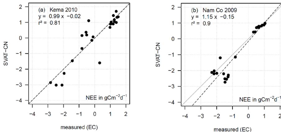
Figure D4. Comparison of hourly medians (see Fig. D3) of measured and modelled net ecosystem exchange for the 2010 campaign at Kema (left panel) and 2009 campaign at Nam Co (right panel). The regression line (dashed, black) is shown as well as the 1 : 1 line (solid, gray).
