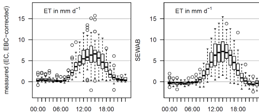
Figure D2. Mean diel course of measured and energy balance corrected evapotranspiration ET (left panel) and SEWAB modelled ET (Tile approach according to the EC footprint: S_{RefEC} , right panel) over 61 days of 2010 (3 June to 2 August) at Kema: box plot with median, 25% and 75% quartiles; bars represent quartiles \pm 1.5 times interquartile range, dots are outliers. Measured and modelled values are restricted to high flux data quality (flag 1–3). Measured data is corrected according to the surface energy imbalance with the buoyancy flux correction.
