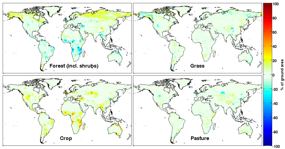
Fig. 2. Figure 1-2: Vegetation changes between 2006 and 2100 for RCP 2.6.
