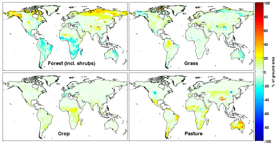
Fig. 4. Figure 1-4: Vegetation changes between 2006 and 2100 for RCP 8.5.
