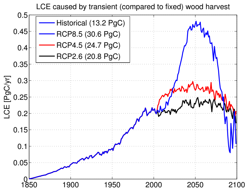
Fig. 1. Figure 1-1: LCE contribution from wood harvest.
