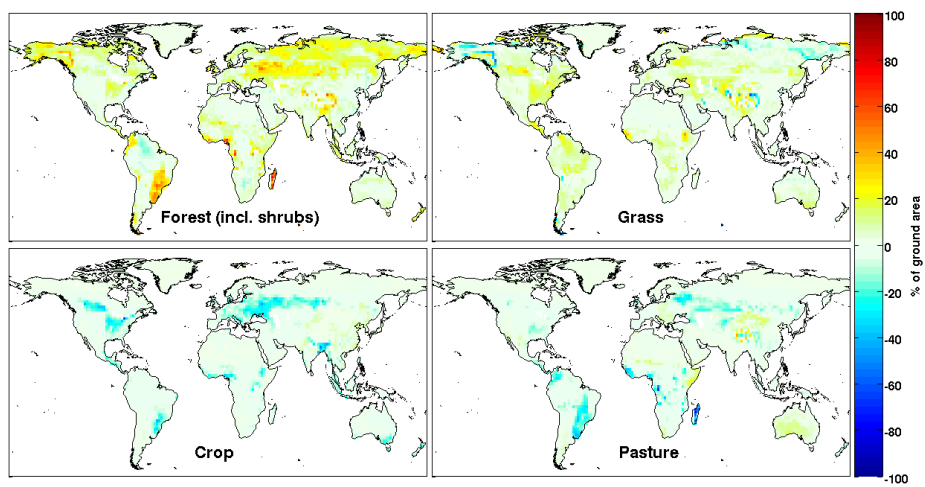
Fig. 3. Figure 1-3: Vegetation changes between 2006 and 2100 for RCP 4.5.
