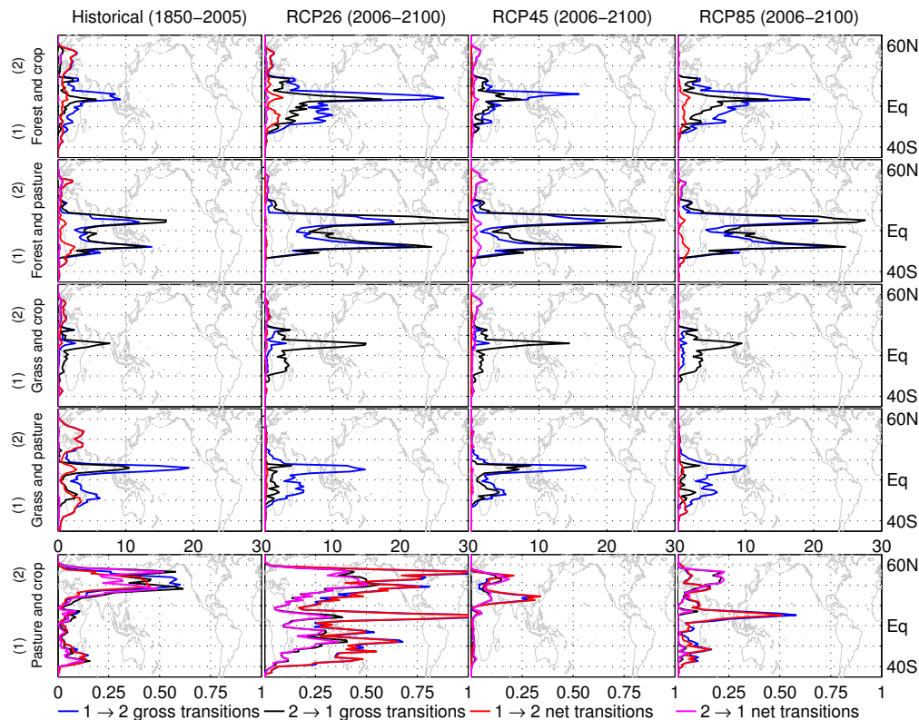
Fig. 3. Figure 3-3: Yearly average land-use changes [ 10^3 \text{ km}^2/\text{latitude band}/\text{yr} ]. [Full caption in text].
