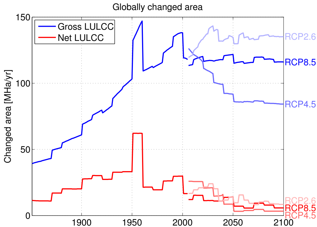
Fig. 2. Figure 3-2: Time series of annual vegetation areas converted by LULCC for the used scenarios.
