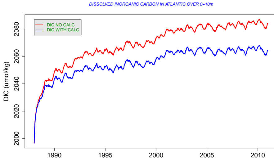
Figure 2: Sea surface DIC in the Atlantic ocean from the reanalysis run, when the \text{CaCO}_3 cycle is included (blue line), or not (red line).
