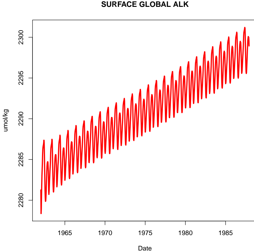
Figure 3: Surface alkalinity during spinup, averaged over the global ocean area.
