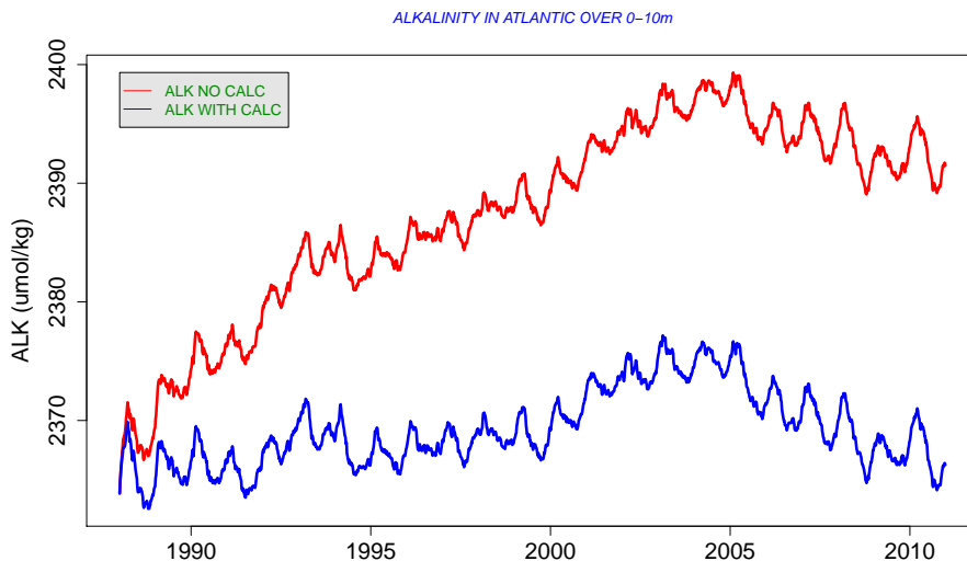
Figure 1: Sea surface alkalinity in the Atlantic ocean from the reanalysis run, when \text{CaCO}_3 cycle is included (blue line), or not (red line).
