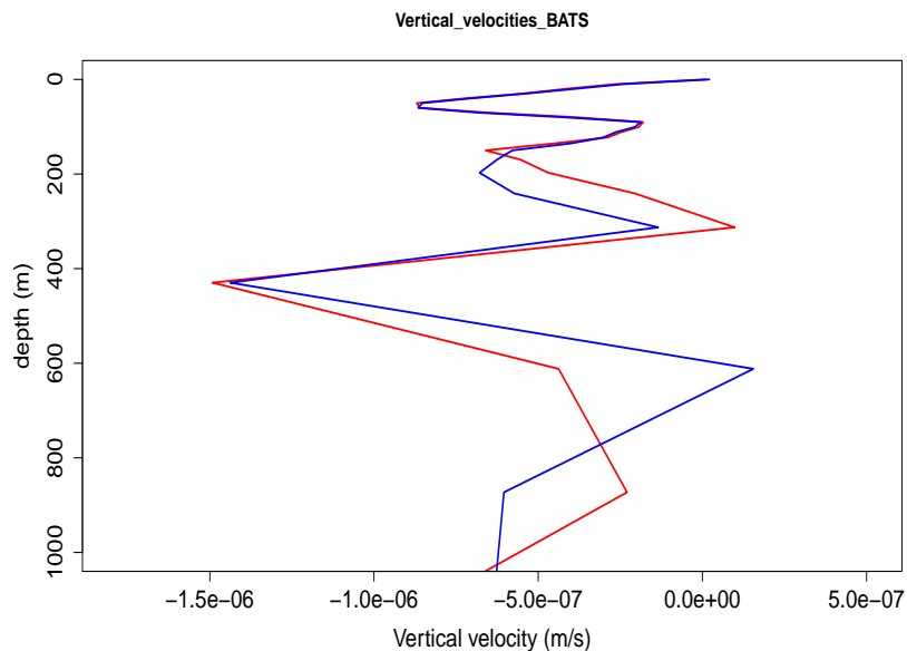
Figure 2: Averaged vertical velocity at BATS for CTRL (blue) and TSREAN (red).
