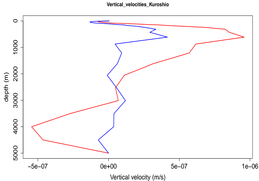
Figure 1: Averaged vertical velocity in the region for CTRL (blue) and TSREAN (red).
