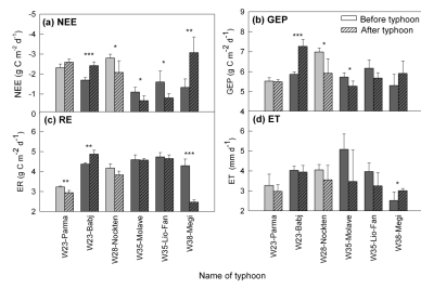
Fig. 4. Average daily (a) net ecosystem CO 2 exchange (NEE), (b) gross ecosystem production (GEP), (c) ecosystem respiration (RE), and (d) evapotranspiration (ET) before and after six typhoons made landfall. Dark grey bars represent the values during the typhoons occurred at Yunxiao, and light grey bars are for those during the typhoons occurred at Gaoqiao.
