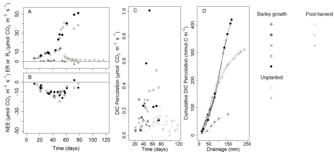
Fig. 2. Gaseous and dissolved CO 2 fluxes from mesocosms.
