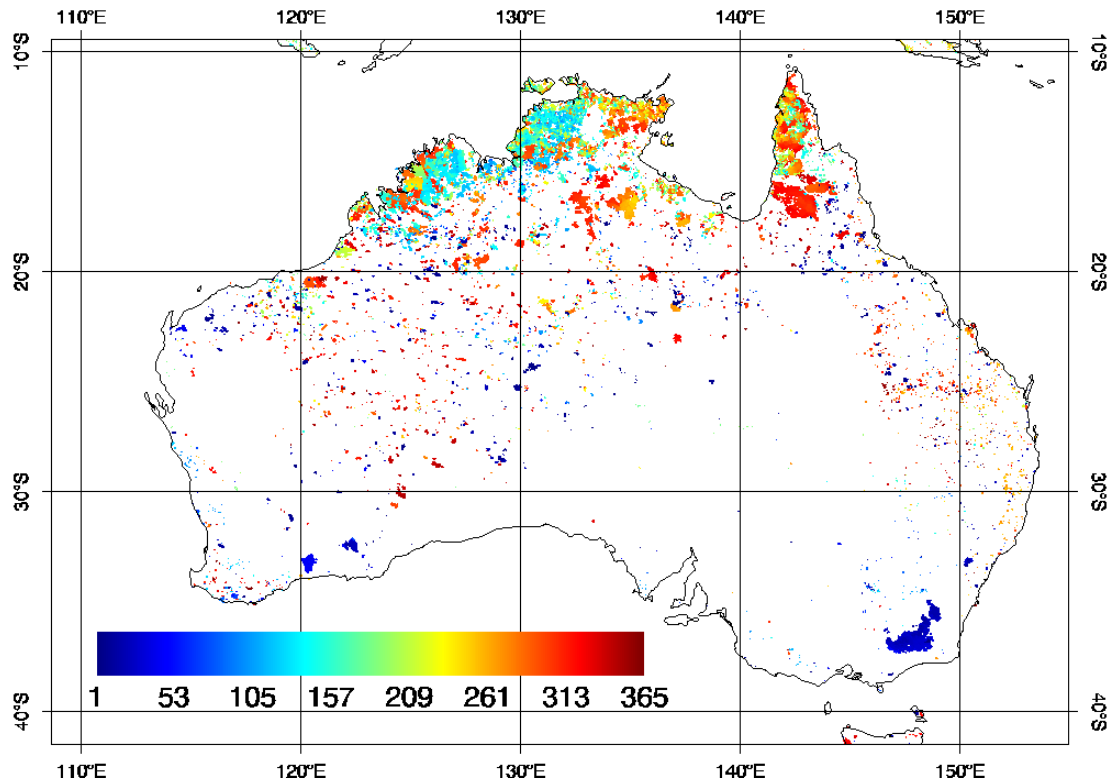
Fig. 4. Figure 3. DoB for Australia during 2003
