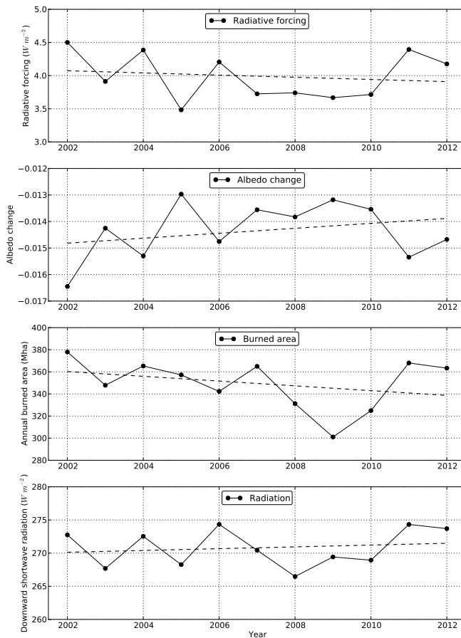
Fig. 3. Figure 2. Temporal changes of the annual global radiative forcing induce by fires and albedo change spanning from 2002 to 2012. Bottom plots show the total annual burned area and the downward SW
