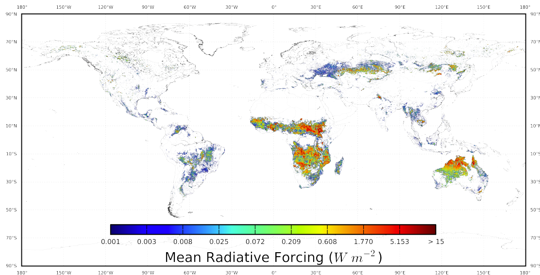
Fig. 1. Figure 1. Global mean radiative forcing caused by “instantaneous” shortwave albedo changes on areas affected by fires. The values were normalized using a logarithmic scale.
