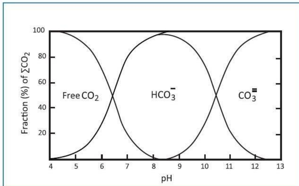
Fig. 1. DIC species vs. pH graph
