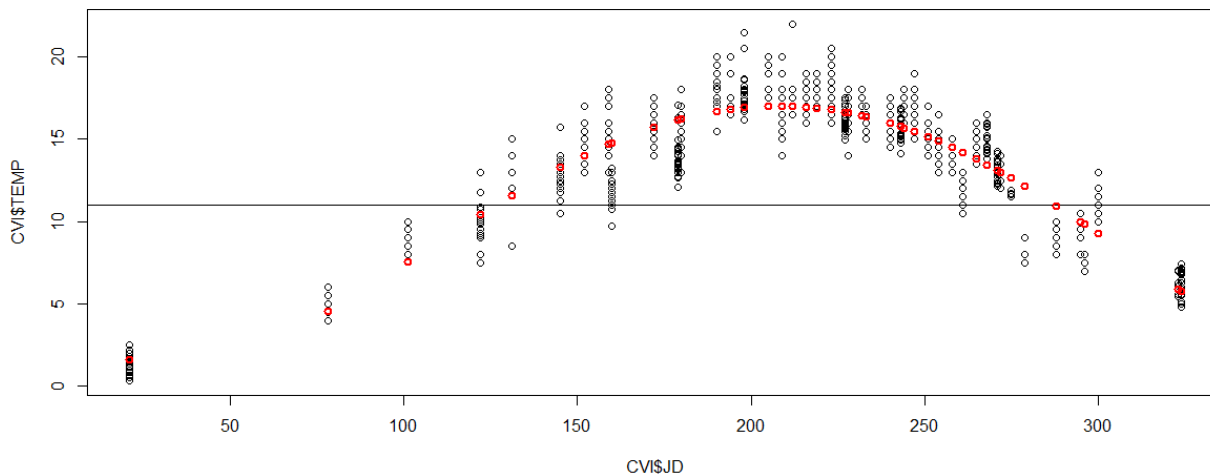
Figure 1. Soil temperature at 12 cm (°C) against Julian Day. The black circles indicate plot level measurements of soil temperature, while the red circles indicate fitted values from our fourth-order polynomial.
