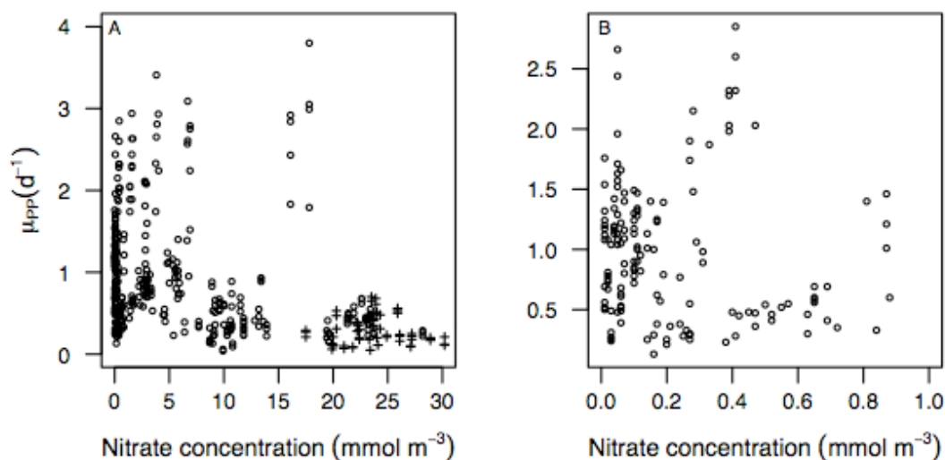
“Figure 6. Relationships between in situ community growth rates ( \mu_{PP} , d^{-1} ) estimated
