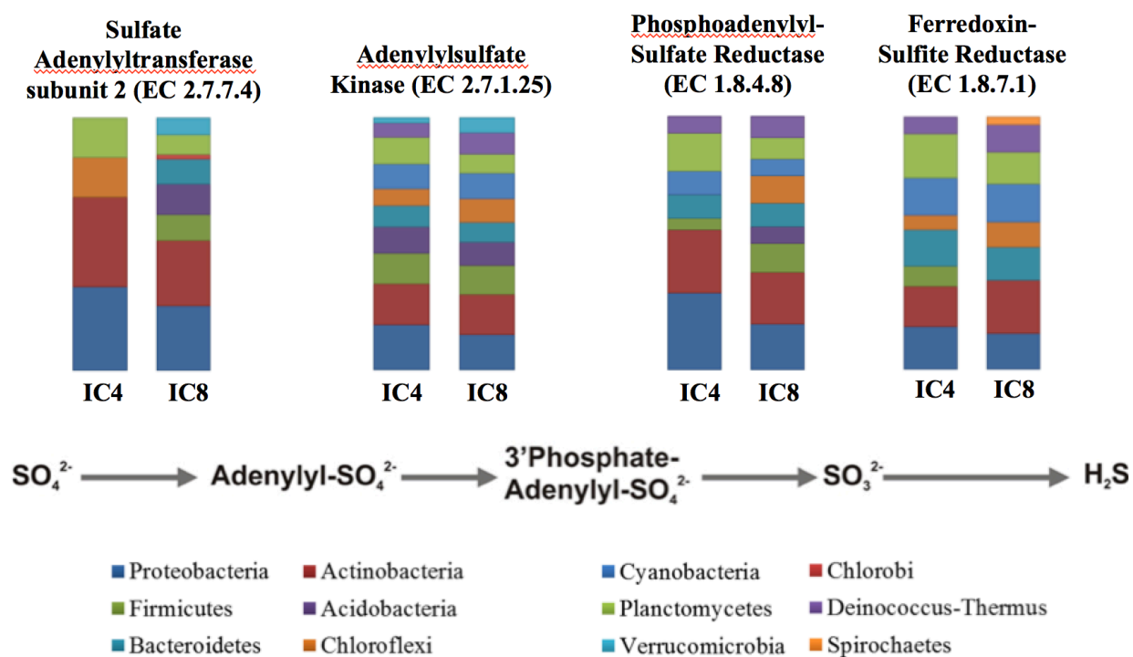
Fig. 6. Phylogenetic distribution of the sequences related to sulfur metabolism (sulfur reduction) within the IC4 and IC8 metagenomes.
