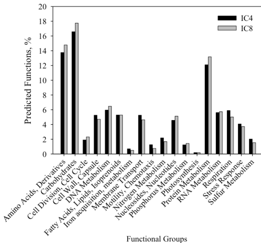
671 Fig. 3. Percentage of gene sequences associated with different functions in the annotated protein 672 sequences within IC4 and IC8 metagenomes.
