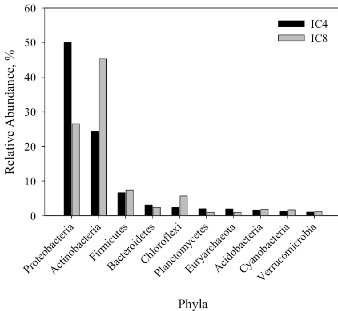
667 668 Fig. 2. Community analyses of the IC4 and IC8 metagenomes at phylum level. The phyla present in 669 metagenomes at a >1% level are shown.
