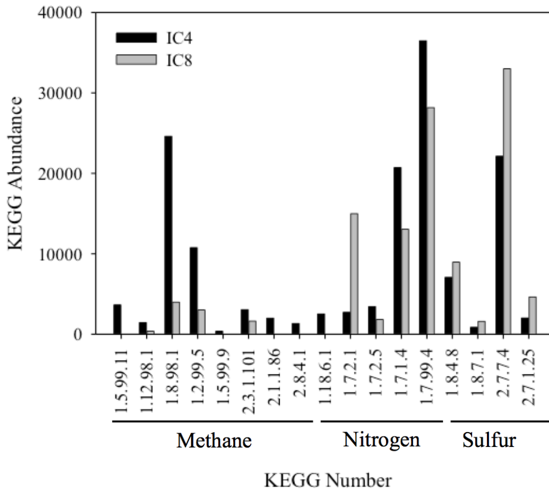
674 Fig. 4. KEGG abundance of the selected functional gene sequences found within IC4 and IC8 675 metagenomes. Genes found in low abundance were not included in the figure. Genes from methane, 676 nitrogen, and sulfur metabolic pathways are underlined. The enzyme name that corresponds to each 677 KEGG number is given in Table 2.
