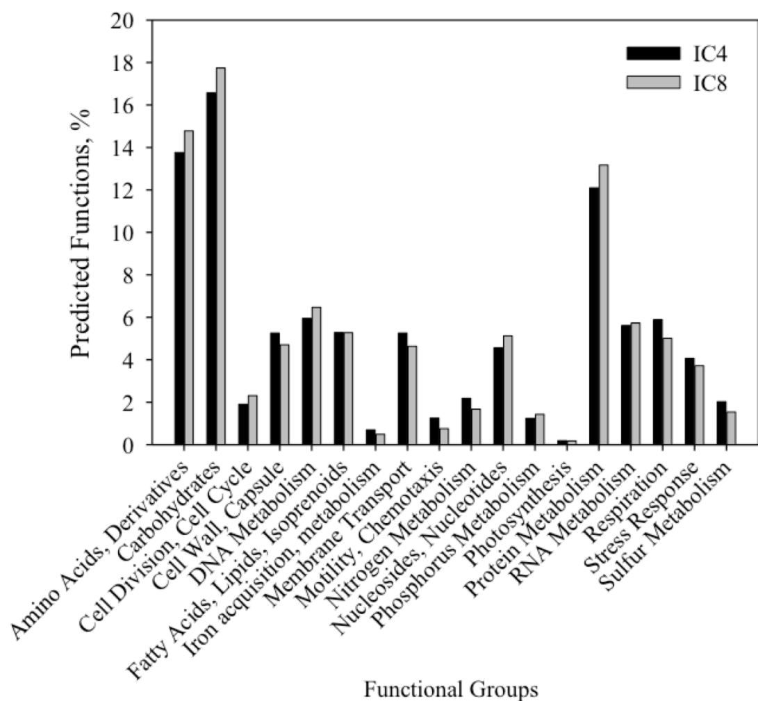
779 Fig. 3. Percentage of gene sequences associated with different functions in the annotated protein 780 sequences within IC4 and IC8 metagenomes.
