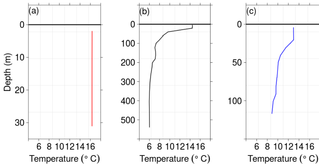
Figure 2. Temperature profiles as recorded by a CTD cast for: (a) Station 11 (SNS); (b) Station 65 (SKNT); (c) Station 80 (NNS)
