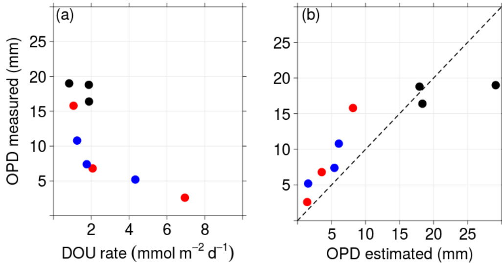
Figure 7. (a) Oxygen Penetration Depth (OPD) plotted versus Diffusive Oxygen Uptake (DOU) rate (b) Correlation between measured OPD and theoretical OPD. Dashed line: 1:1 line; Red symbols: SNS; Blue symbols: NNS; Black: SKNT. For calculation and details see text.
