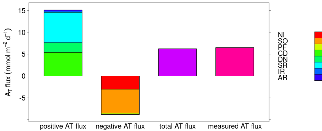
Figure 12. Contribution of different processes to the benthic A_T budget in the SNS. For more details on different reaction rates see text. NI: Nitrification; SO: Sulfide oxidation; PF: Pyrite formation; CD: Carbonate dissolution; DN: Denitrification; SR: Sulfate reduction; IR: Dissimilatory iron reduction; AR: Aerobic respiration. Fluxes in \text{mmol m}^{-2} \text{d}^{-1} .
