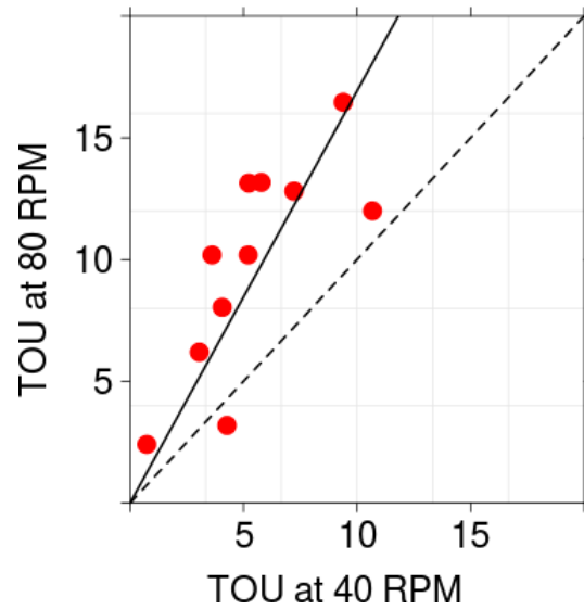
Figure 4. Total oxygen uptake rates measured in benthic incubation chambers at two different stirring rates (RPM = Rounds Per Minute); Dashed line: 1:1 line; Solid line: Linear regression; Red symbols: SNS. All rates in \text{mmol O}_2 \text{ m}^{-2} \text{ d}^{-1} .
