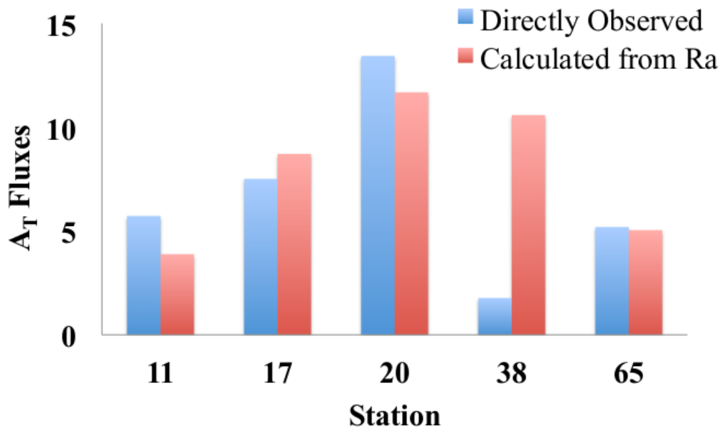
Figure 10. Directly measured A_T fluxes for the SNS compared to A_T flux estimations based on Ra measurements. Figure taken from Burt et al. (2014). Fluxes in mmol C m -2 d -1 .
