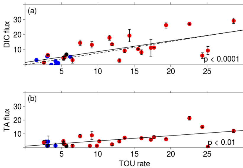
Figure 8. (a) Correlation between DIC fluxes and TOU rates. (b) Correlation between A_T fluxes and TOU rates. Solid line: Linear regression; Spearman's p -value given in each plot. TA and DIC fluxes in mmol C m -2 d -1 . TOU rates in mmol O 2 m -2 d -1 .
