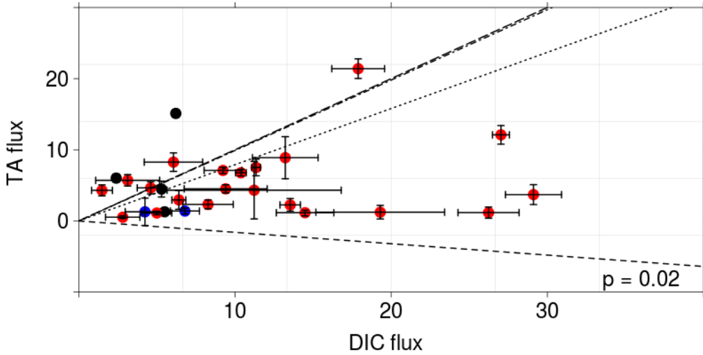
Figure 11. Correlation between A_T and DIC fluxes for sites of the SNS from both campaigns. Different lines are representing different reaction stoichiometry. For more explanation and reaction equations s. text. Short dashed line: Aerobic respiration; Dotted line: Denitrification; Dotted/Dashed line: Sulfate reduction coupled to pyrite formation and burial; Long dashed line: Carbonate dissolution; Note, that the latter two lines are plotting along similar points and are thus hard to distinguish. p: Spearman's rank correlation coefficient for the correlation of all points displayed in this scatter plot. All fluxes in \text{mmol C m}^{-2} \text{d}^{-1} .
