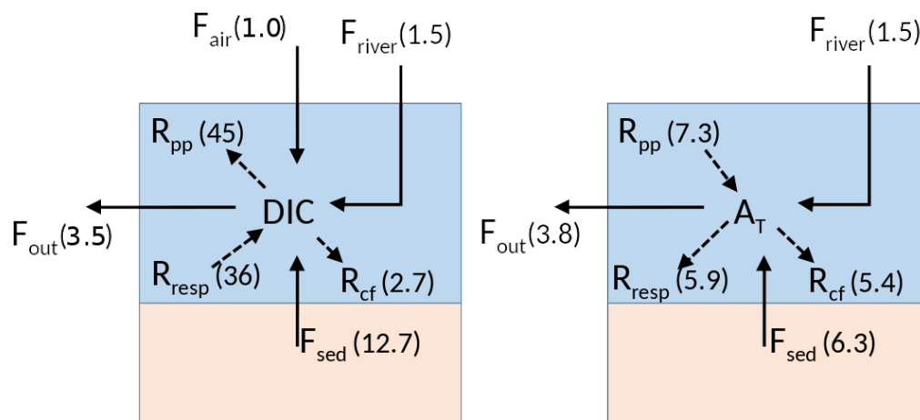
Figure 13. DIC and A_T budgets of the water column in the SNS. Bold arrows: Fluxes; Dashed arrows: Reaction rates. F_{sed} : Net flux from the sediments; F_{river} : Riverine input; F_{out} : Flux into the NNS/SKNT; F_{air} : Atmospheric DIC uptake; R_{pp} : Primary production rate; R_{resp} : Aerobic respiration rate; R_{cf} : Carbonate production rate. Unit: \text{mmol C m}^{-2} \text{d}^{-1}
